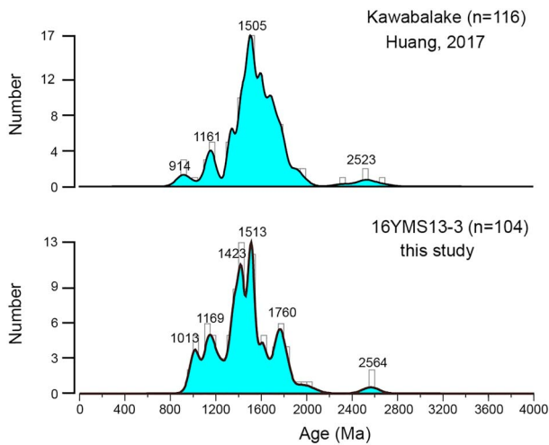
Figure 13. Normalized kernel density plot curves for detrital zircon ages in the quartz arenite cobble in this study and a sandstone from the Kawabalake Group of the Central Tianshan Arc (Huang, 2017).
