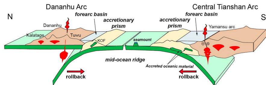
Figure 14. Schematic diagrams illustrating the tectonic evolution of the North Tianshan Ocean and adjacent areas. (a) Cambrian-Ordovician subduction of the North Tianshan Ocean generated the Dananhu Arc in the north and built the Central Tianshan Arc above a Precambrian basement in the south; (b) During the Silurian-Late Devonian, the North Tianshan Ocean continued its two-way subduction; (c) During the latest Carboniferous-Permian, southward subduction and rollback of the North Tianshan Ocean gave rise to the magmatism in the Yamansu Arc. The North Tianshan Ocean terminated along the Kangurtag belt. KOF = Kangurtag ophiolite fragments (see text for details).
