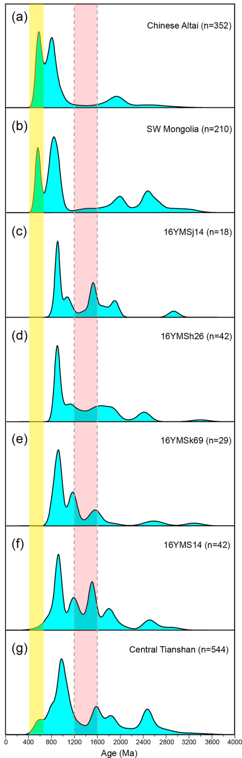
Figure 12. Normalized kernel density plot curves for detrital zircon ages of samples analyzed in this study and those of Paleozoic sandstones from the Chinese Altai (Jiang et al., 2011; Long et al., 2007; Long et al., 2010; Wang et al., 2014), SW Mongolia (Gibson et al., 2013; Jiang et al., 2012; Rojas-Agramonte et al., 2011), and the Central Tianshan Arc (see text for details). Only Precambrian ages are plotted.
