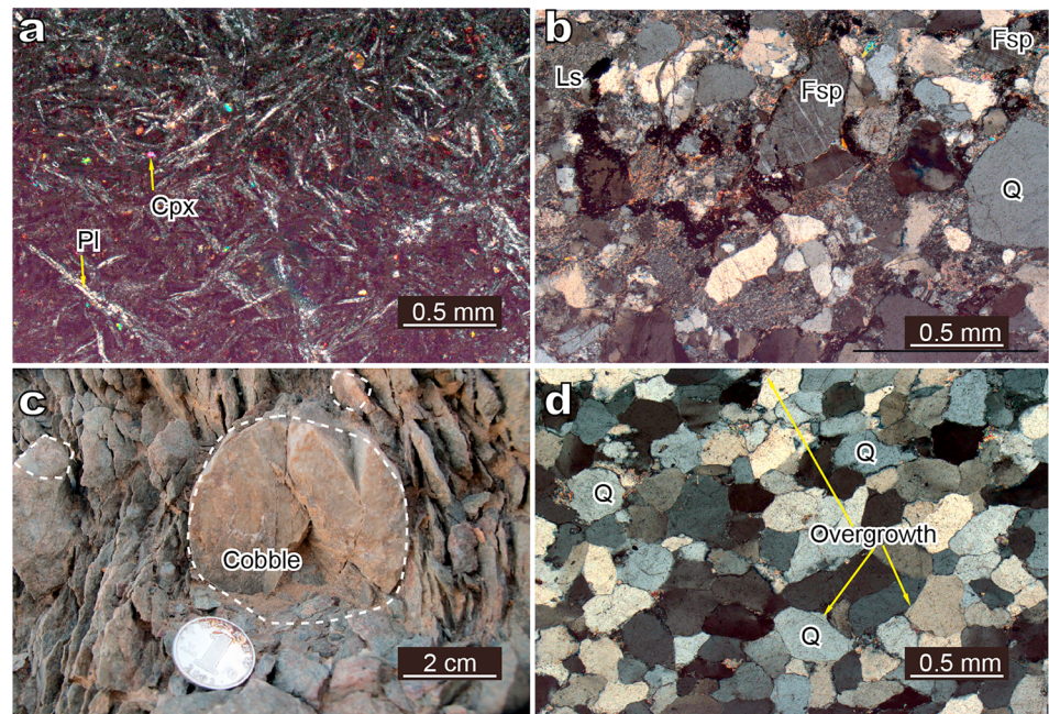
Figure 6. Photos of representative samples from the Southern Kangurtag mélangé. (a) Photomicrograph of pillow basalts. (b) Photomicrograph of feldspathic greywackes from the Kushui Formation. (c and d) Outcrop and photomicrograph of a quartz arenite cobble from the Kushui Formation. Q = quartz; Fsp = feldspar; Pl = plagioclase; Ls = sedimentary lithic fragment; Cpx = clinopyroxene.
