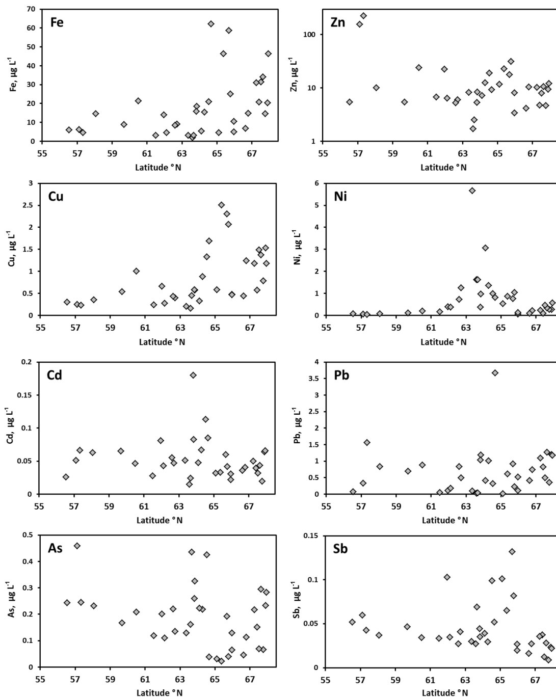
Figure 2. Examples of dissolved ( <0.45\ \mu\text{m} ) metal concentrations in snow water as a function of latitude. The cause for the elevated concentrations of Ni, Cd and Sb at ca. 64\text{--}65^\circ\text{N} is most likely industrial impact, but given relatively low number of data points around industrial centers it is hard to prove it unambiguously.
