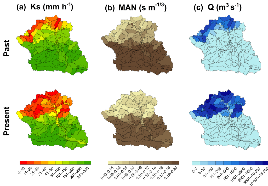
Figure 9. Spatial patterns of the (a) saturated hydraulic conductivity ( K_s ), (b) Manning's roughness coefficient ( Man ) and (c) Discharge ( Q ) between the past and the period for the monsoon season (JAS).
