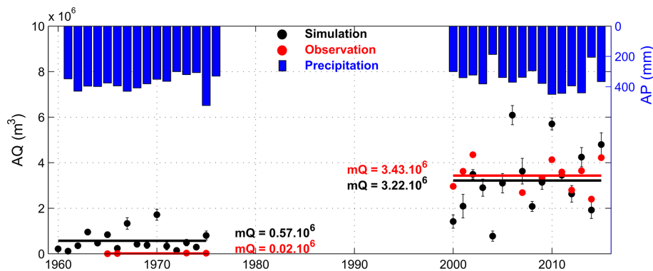
Figure 6. Evolution of annual discharge (AQ, in \text{m}^3 ) between 1960 and 2015: simulations with standard deviation of the 10 members (black dots with error bar) and observations (red dots) together with annual precipitation (AP, in mm, blue bars).
