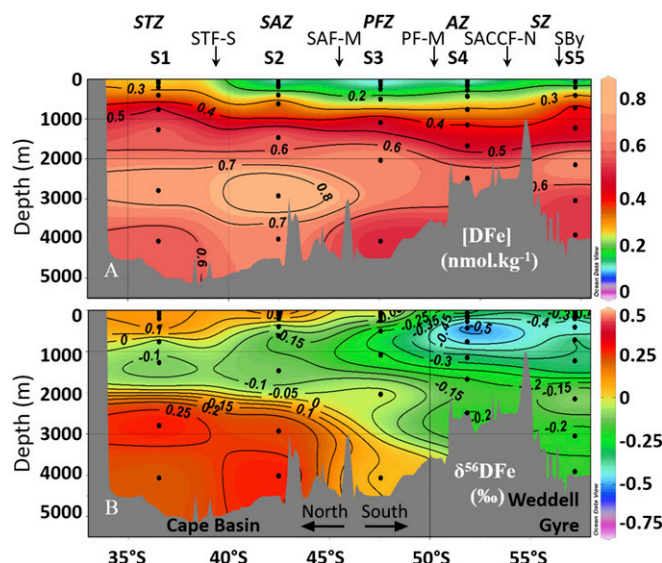
Fig. 4. Sections of (A) DFe concentrations ( [\text{DFe}] in nanomoles per kilogram) and (B) DFe isotopic composition ( \delta^{56}\text{DFe} relative to IRMM-14 in per mill) of seawater samples taken during the BGH cruise (black dots). Fronts locations are indicated. See Fig. 2 for acronyms. Figure was made using Ocean Data View (55).
