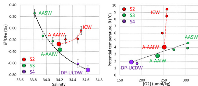
Fig. 5. Mixing diagrams. Properties of the Drake Passage Upper Circumpolar Deep Water (DP-UCDW), Atlantic Antarctic Intermediate Water (A-AAIW), Antarctic Surface Waters (AASW), and Indian Central Water (ICW) are shown for stations S2, S3, and S4. The dotted lines denote the theoretical conservative mixing curves between DP-UCDW and AASW (black dotted line) and A-AAIW and ICW (red dotted line; see Supporting Information for the mixing equations). The large symbols identify the \delta^{56}\text{DFe} minimum sample at each station. The diagrams show that the A-AAIW properties can be explained by a mixing between DP-UCDW and AASW. The slight deviation of the S2 A-AAIW properties from this mixing (black dotted line) is explained by a small contribution of the warm and salty Indian Central Water (red).
