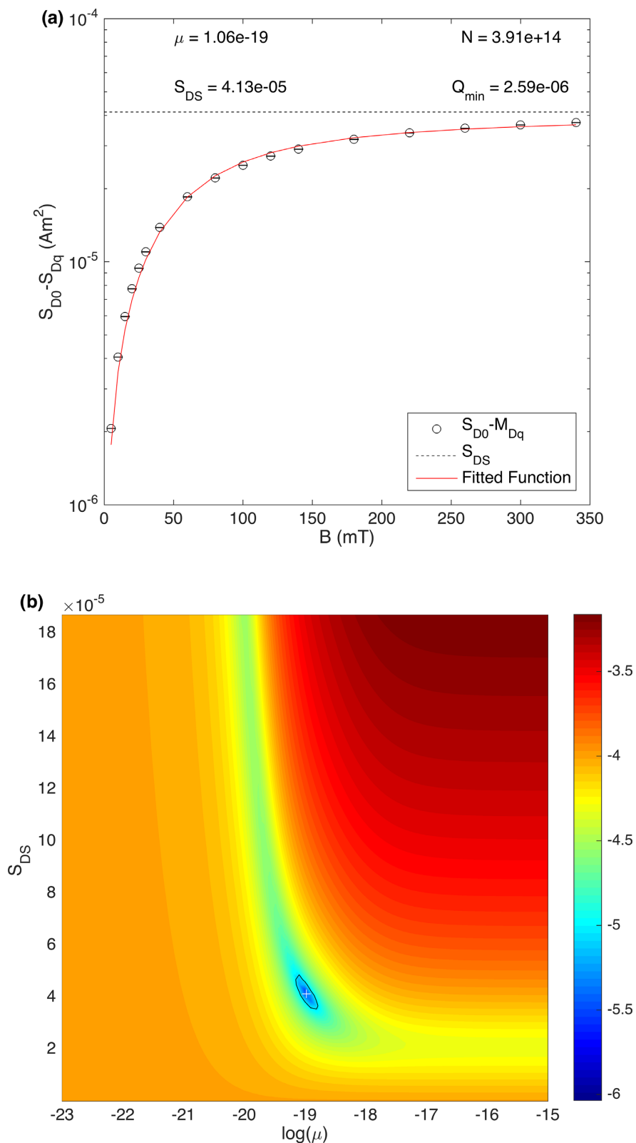
Figure 4. Inversion products of the SPCDM procedure; (a) data fitting and estimated parameters grain dipole moment \mu [Am 2 ]; sample dipole saturation S_{DS} [Am 2 ] and number of magnetic carriers N . Measured data (black circles) and fitting curve (red) from the inverted model parameters. (b) Objective function with inverted model solution (white cross). For the sake of graphical representation the value of 10 \varepsilon is contoured (black) for a threshold data fitting \varepsilon equal to 5.0E-8 , with stop criterion Q_{min} < \varepsilon .
