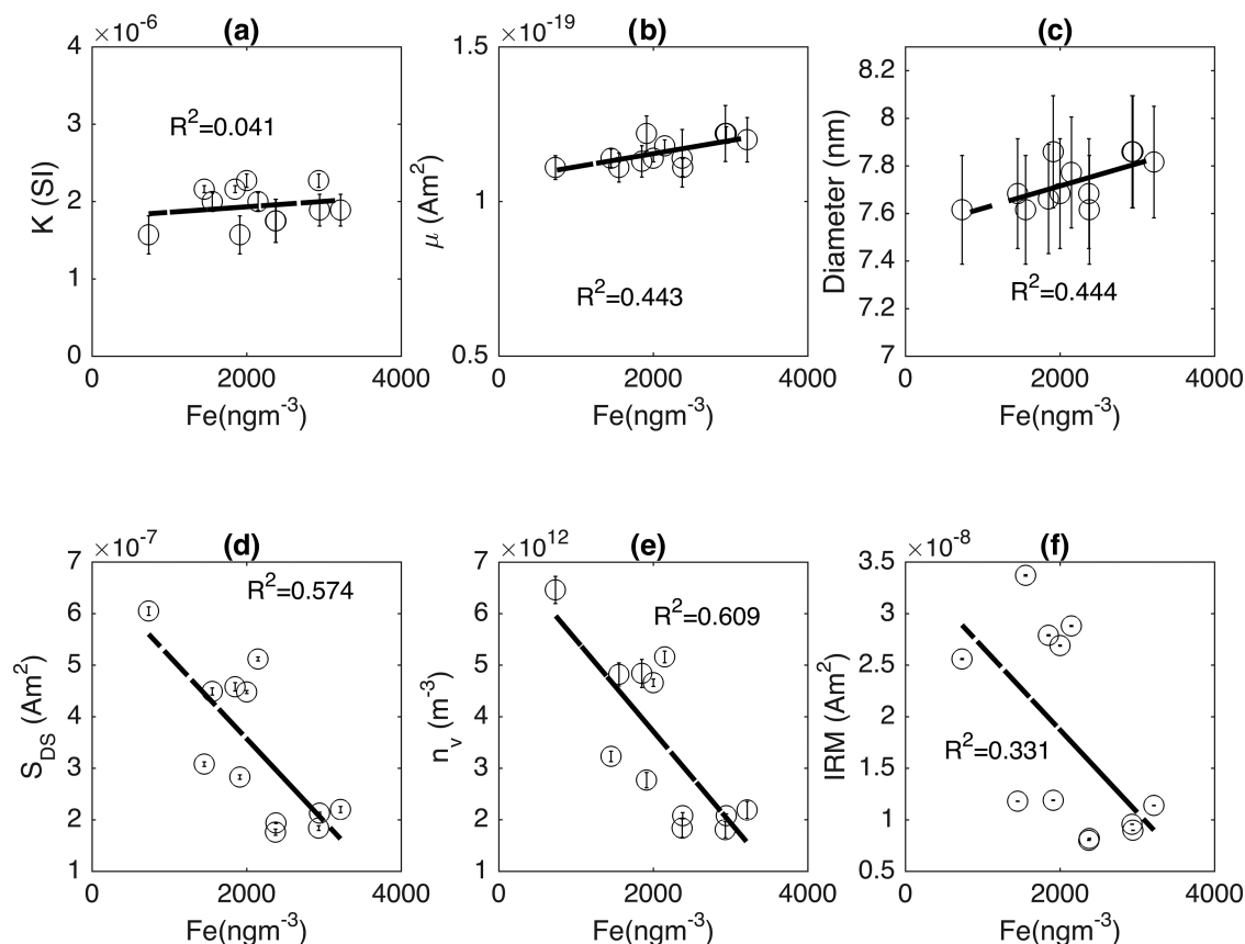
Figure 7. SPCDM results and magnetic properties for air PM collected in Jânio Quadros tunnel in São Paulo.
