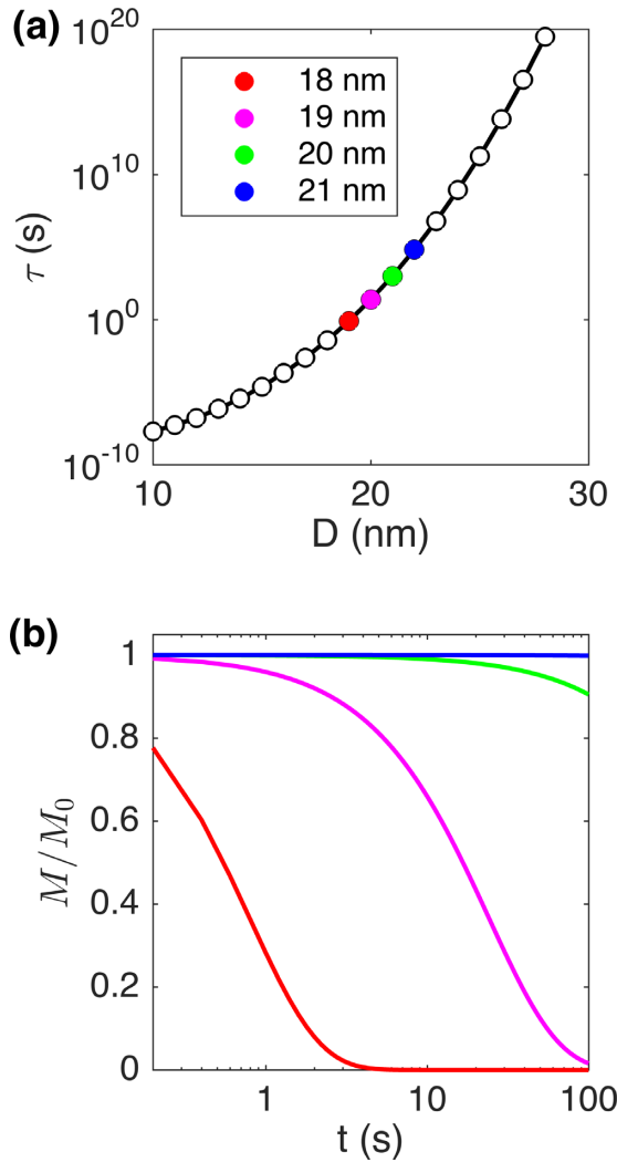
Figure 1. (a) Variations of relaxation time with diameter of spherical magnetite-like minerals and (b) corresponding magnetization decay normalized by initial magnetization M_0 . Blocking volume with stable magnetization (blue), thermally active particles with viscous (green and magenta) and fast (red) magnetic relaxation as expected in 100 s window.
