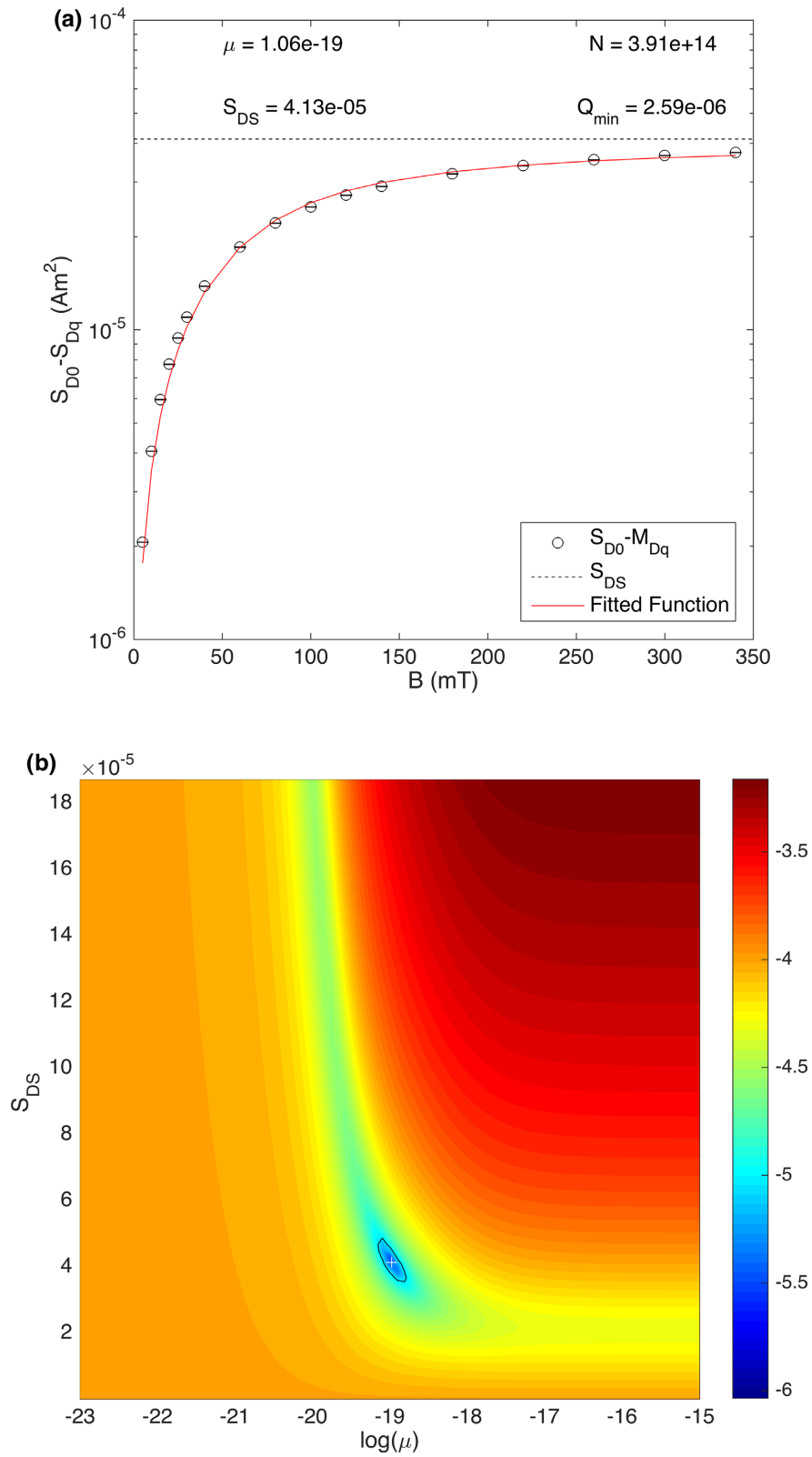
Figure 4. Inversion products of the SPCDM procedure; (a) data fitting and estimated parameters grain dipole moment \mu [ \text{Am}^2 ]; sample dipole saturation S_{DS} [ \text{Am}^2 ] and number of magnetic carriers N . Measured data (black circles) and fitting curve (red) from the inverted model parameters. (b) Objective function with inverted model solution (white cross). For the sake of graphical representation the value of 10 \varepsilon is contoured (black) for a threshold data fitting \varepsilon equal to 5.0\text{E-}8 , with stop criterion Q_{\min} < \varepsilon .
