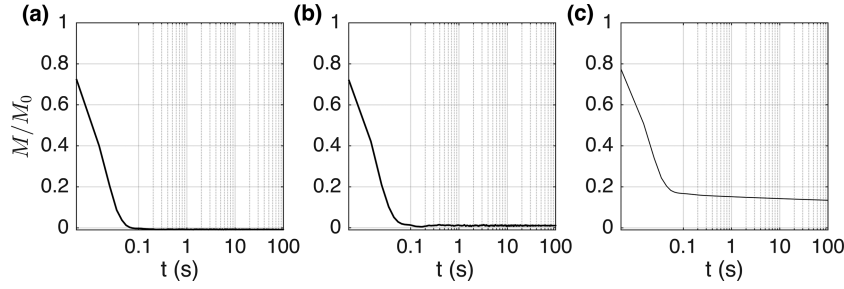
Figure 3. Magnetization relaxation after applying a 500 mT normalized by in field magnetization M_0 ; (a) nanoparticle of synthetic magnetite with fast relaxation; (b) air particulate matter with same behaviour and (c) sediments from Jaraguá Cave with slower magnetization decay, suggestive of coarser SP minerals.
