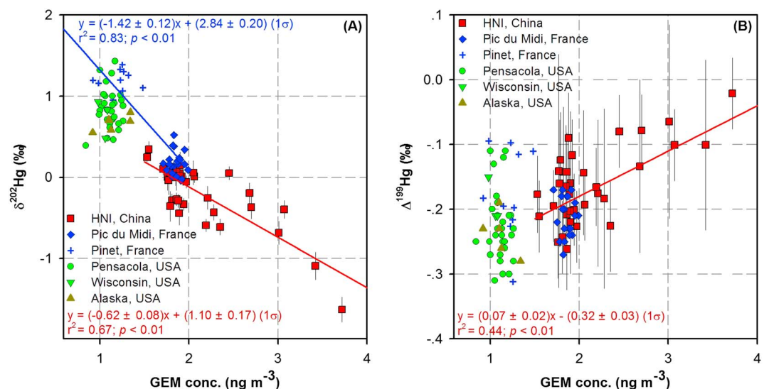
Figure 3. Relationship between atmospheric GEM concentrations and (a) GEM \delta^{202}\text{Hg} and (b) GEM \Delta^{199}\text{Hg} (error bars on GEM \delta^{202}\text{Hg} and \Delta^{199}\text{Hg} indicates 2\sigma uncertainty) in this study, Europe, North America, and Arctic. Data are from this study and the literature (Demers et al., 2013, 2015; Enrico et al., 2016; Fu, Maruszczak, Wang, et al., 2016; Obrist et al., 2017).
