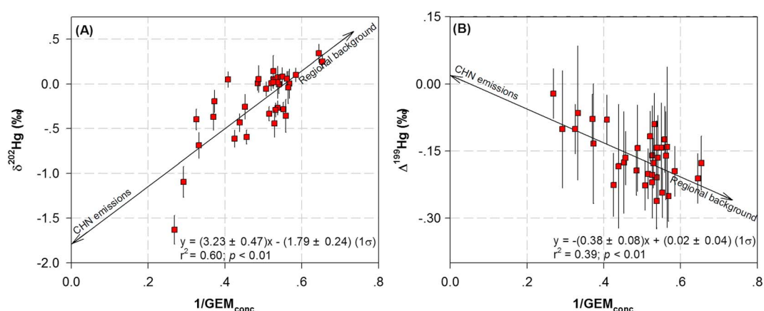
Figure 4. (a) \delta^{202}Hg versus 1/GEM and (b) \Delta^{199}Hg versus 1/GEM diagrams suggesting a binary mixing of regional background atmospheric GEM pool and Chinese (CHN) emissions of GEM.
