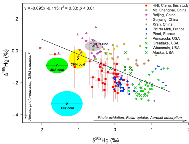
Figure 2. Mass-dependent ( \delta^{202}\text{Hg} ) and mass-independent ( \Delta^{199}\text{Hg} ) isotope signatures of atmospheric TGM/GEM and source materials (e.g., China, United States, and European feed coal and China zinc ores) worldwide. The error bar on \delta^{202}\text{Hg} and \Delta^{199}\text{Hg} of atmospheric GEM at HNI and source materials indicates 2\sigma and 1\sigma of isotopic measurement, respectively. The black line represents the relationship between GEM \delta^{202}\text{Hg} and \Delta^{199}\text{Hg} for the global observations. Data are from this study and the literature (Demers et al., 2013, 2015; Enrico et al., 2016; Fu, Maruszczak, Wang, et al., 2016; Fu, Zhu, et al., 2016; Gratz et al., 2010; Lefticariu et al., 2011; Obrist et al., 2017; Sun et al., 2014; Yin et al., 2014, 2016; Yu et al., 2016).
