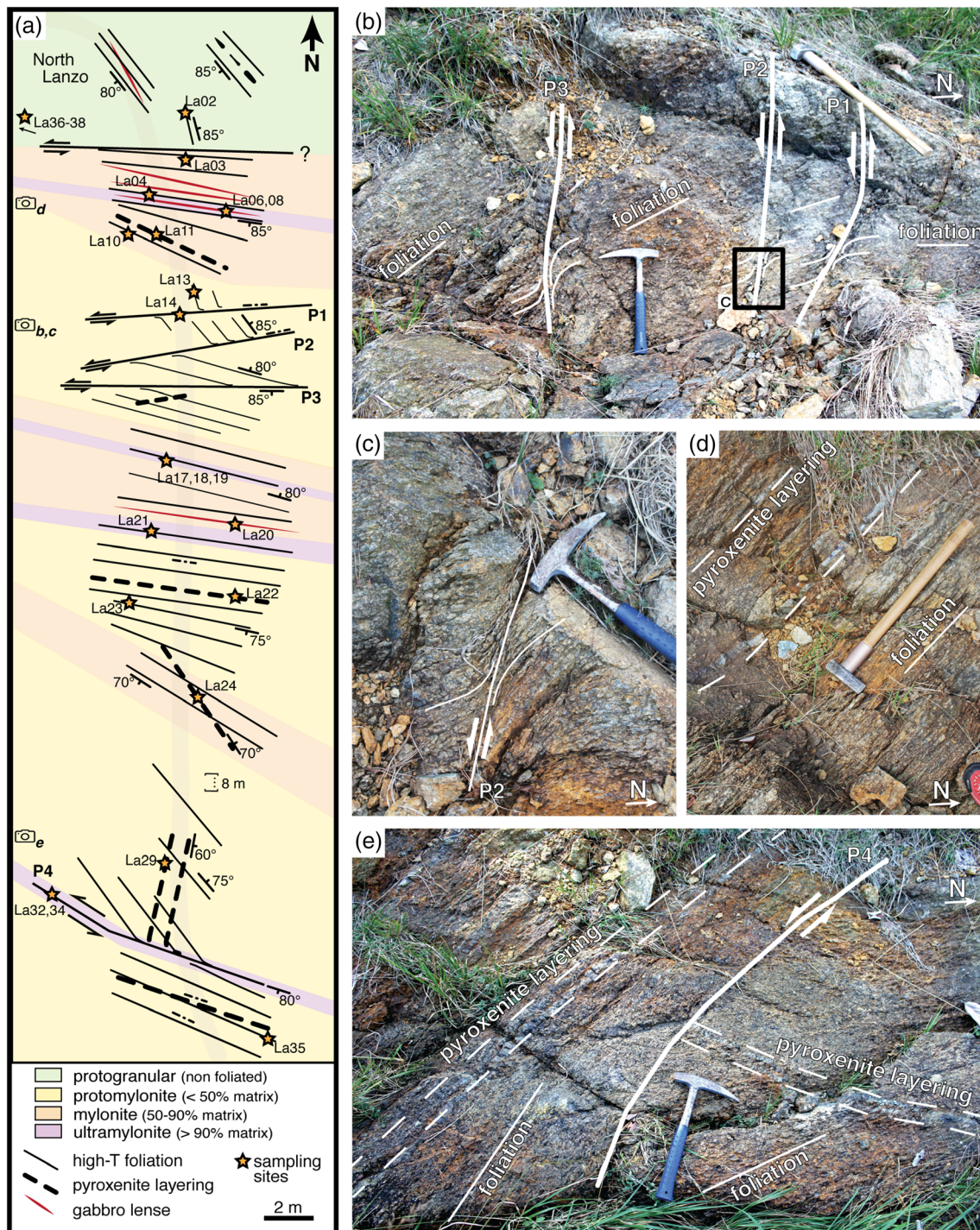
Figure 2. Geological map and structures of the hydrous mylonite zone. (a) Detailed structural map of the selected outcrop (~50 m long), with reference to the different textural types. Shear senses are indicated by arrows. The boundary between the northern and central Lanzo domains is possibly defined by the fault delimiting the protogranular and mylonitic textures at the top of the map. Sampling sites are indicated by yellow stars, and sample description is available in Table 1. (b) Late shear planes affecting the protomylonitic peridotite (P1–P3). (c) Drag fold associated with shear plane P2. (d) Mylonite showing the subparallel relationship between pyroxenite bands and high-temperature foliation. (e) Discordant pyroxenite bands and high-temperature foliation on either side of shear plane P4. Drag folds associated with P4 are only 1 cm in size.
