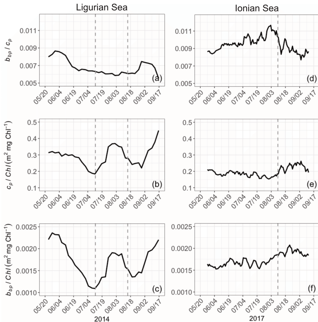
Figure 9. Temporal evolution of the bio-optical ratios of b_{bp}/c_p (a), c_p/Chl (b) and b_{bp}/Chl (c) in the SCM layer for the Ligurian Sea (a–c) and the Ionian Sea (d–f). The dotted lines indicate the dates when the values of c_p in the SCM layer reach a minimum. Please note that the date format in this figure is month/day.
