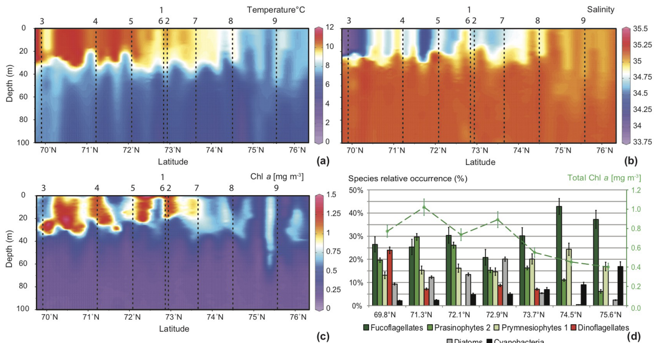
Figure 2. South–north, 0–100 m deep sections across the Barents Sea Opening, compiled from data of the 32 CTD casts: (a) temperature (°C), (b) salinity, and (c) Chl a concentrations ( \text{mg m}^{-3} ). Vertical dashed lines and associated numbers correspond to the location of the MultiNet hauls. The lower right panel (d) displays pigment concentrations translated into the relative abundances of the major phytoplankton species at seven sampling stations along the transect (Giraudeau et al., 2016).
