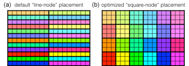
Figure 11. NEMO domain decomposition with the dispatch of the MPI processes among the different nodes. In this schematic representation, each square represents one MPI process of NEMO. We consider that NEMO is distributed over 216 MPI processes and that each node has 9 cores. The distribution of the MPI processes on the cores is represented by their color: processes on the same node have the same color. (a) Default dispatch of the MPI processes in lines; (b) optimized dispatch of the MPI processes in squares.
