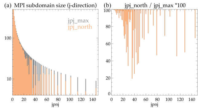
Figure 1. Example of ORCA025 domain decomposition along the j direction (1021 points): (a) j size of the largest MPI subdomains ( jpj_{max} , in grey) and of the northern MPI subdomains ( jpj_{north} , in orange) according to the optimum number of MPI subdomains in the j direction ( jpnj ); (b) ratio jpj_{north}/jpj_{max} in %.
