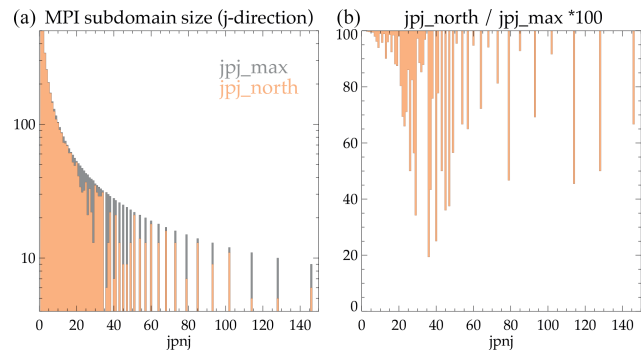
Figure 1. Example of ORCA025 domain decomposition along the j direction (1021 points): (a) j size of the largest MPI subdomains ( jp_{max} , in grey) and of the northern MPI subdomains ( jp_{north} , in orange) according to the optimum number of MPI subdomains in the j direction ( jpnj ); (b) ratio jp_{north}/jp_{max} in %.
