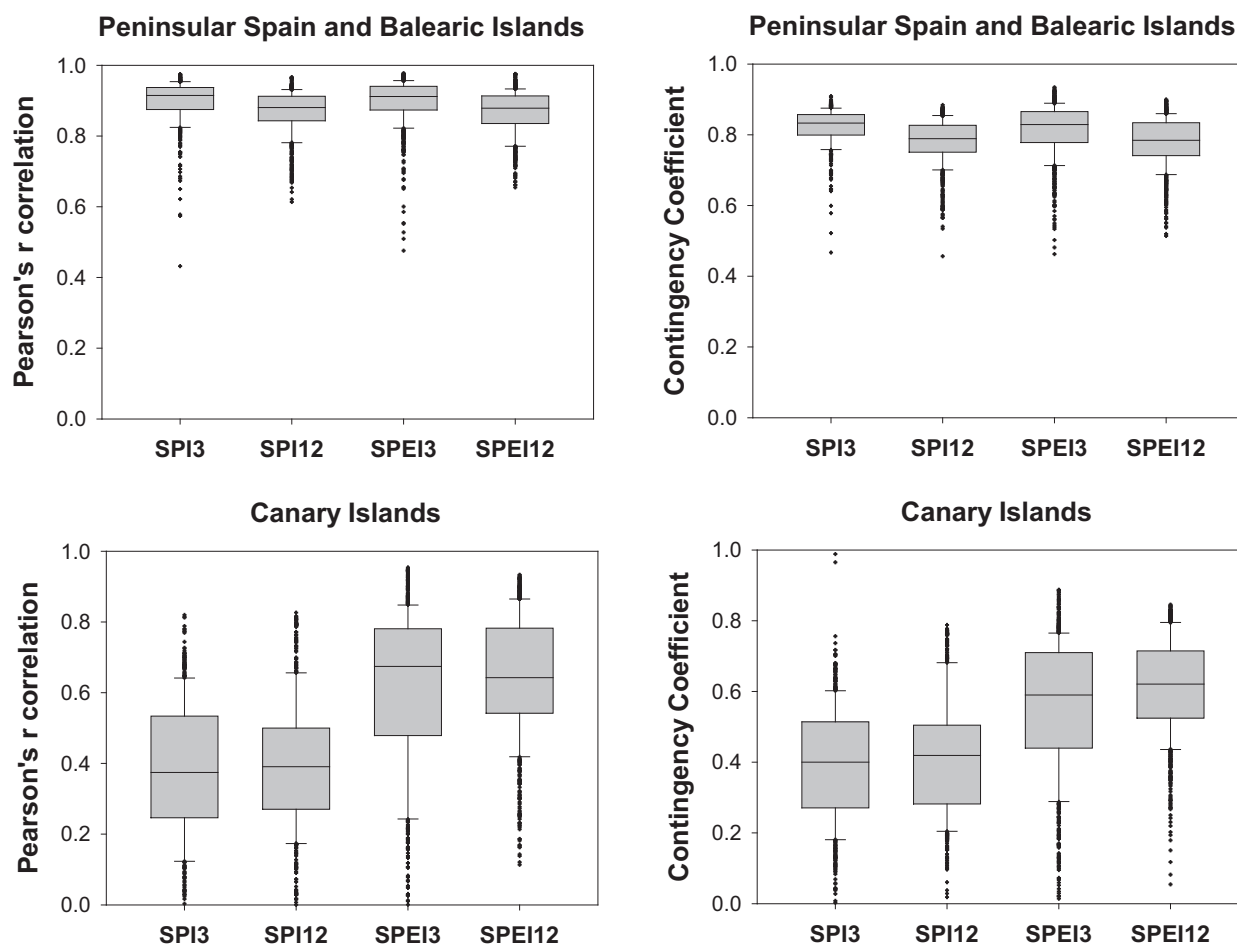
Fig. 11. Left: Box-plots showing the values of Pearson's r correlations between SPI and SPEI series obtained from historical and monitoring datasets in mainland Spain and the Balearic Islands (Top) and the Canary Islands (Bottom). Right: Box-plots showing the coefficients of contingency between different categories of drought (i.e. severe, moderate and mild) calculated from SPI and SPEI series obtained from historical and monitoring datasets in mainland Spain and the Balearic Islands (Top) and the Canary Islands (Bottom).
