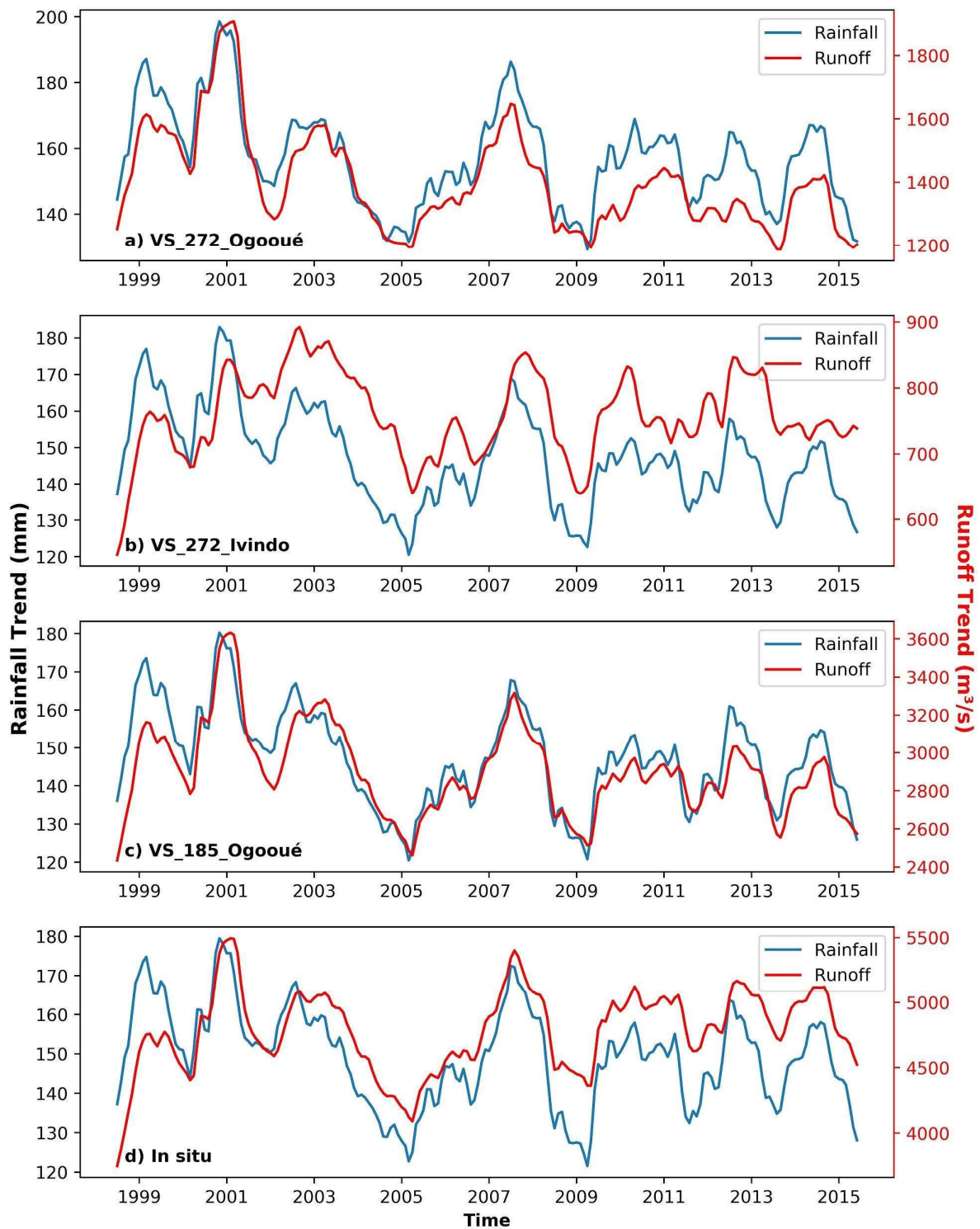
Figure 8: STL decomposition components of rainfall (blue) and river discharge (red) trend components for the four drainage areas of this study.
