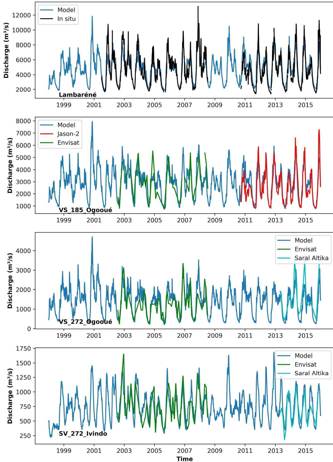
Figure 7: validation of simulated discharges with in situ measured and altimetry derived discharges
