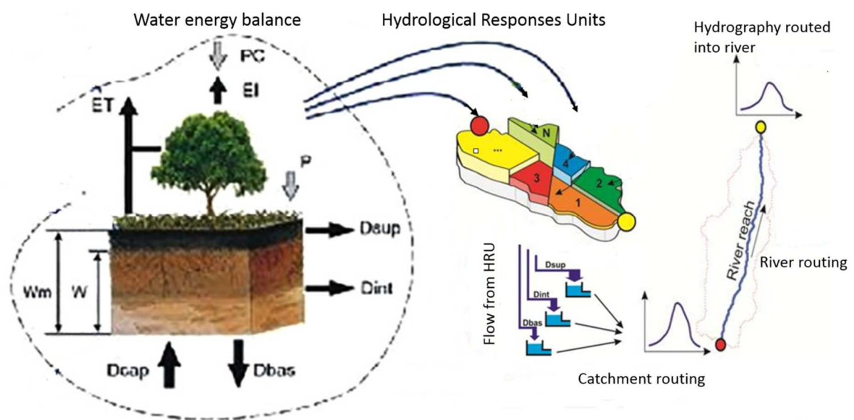
Figure 3: Main processes represented in the MGB model, including PC: precipitation; ET: evapotranspiration; EI: evaporation of intercepted water; P: precipitation discounted by EI; Dsup: surface flow; Dint: subsurface flow; Dbas: groundwater flow; Dcap: capillary flux; W: soil water storage; Wm: maximum soil water storage; E: open water evaporation (source: Siquiera et al. (2018)).
