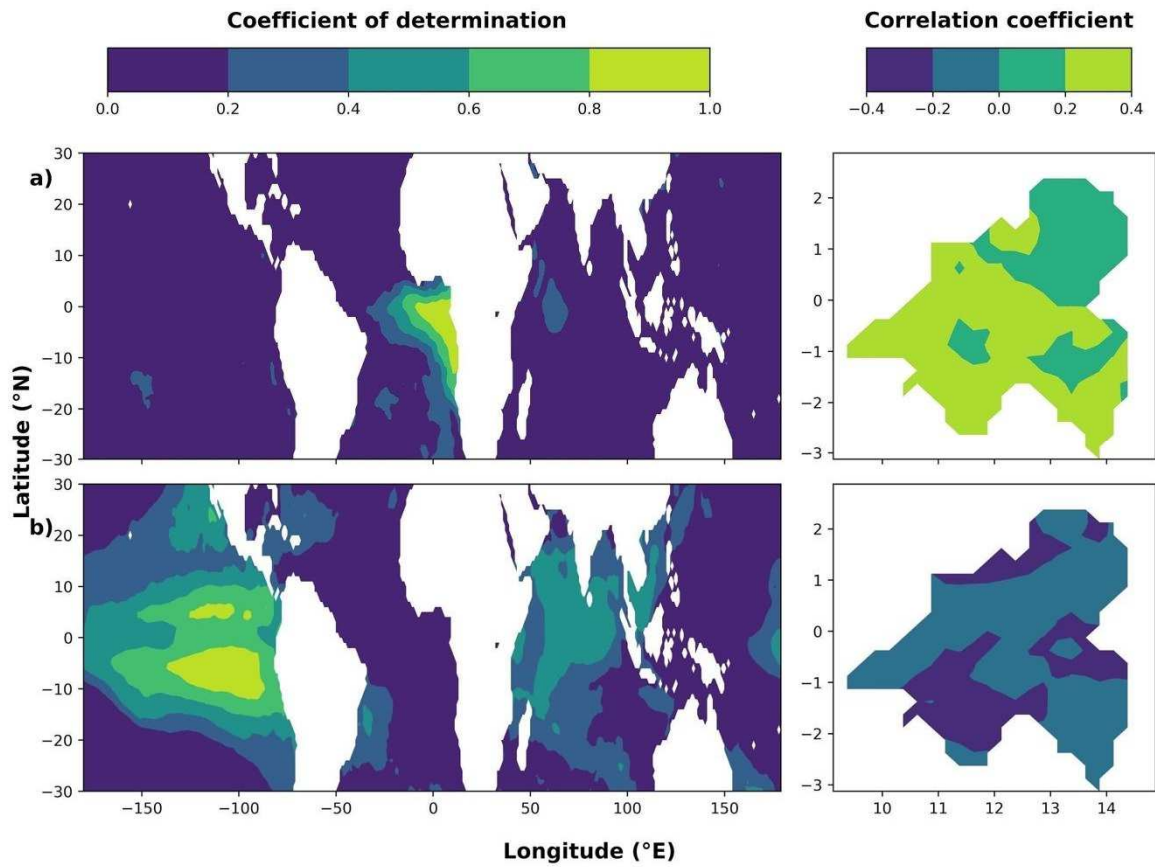
Figure 9: The two first modes of EOT analysis applied in 1998 - 2015 precipitations and 1^\circ \times 1^\circ global tropical SSTs: a) is the first mode and b) is the second mode.
