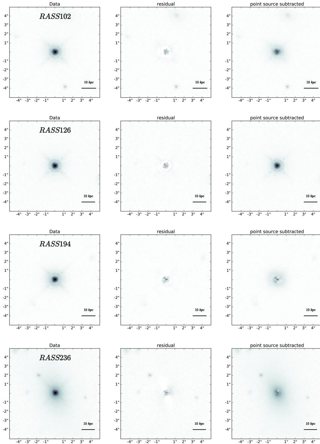
Figure A1. GALFIT host galaxy fits for AGN in this sample, left most column shows raw images, middle column shows residual with full model subtracted, right most column shows residual with point source subtracted. Individual cut-outs are 10 arcsec \times 10 arcsec and are oriented as observed rather than north up and east left to show the similarity in PSF patterns.
