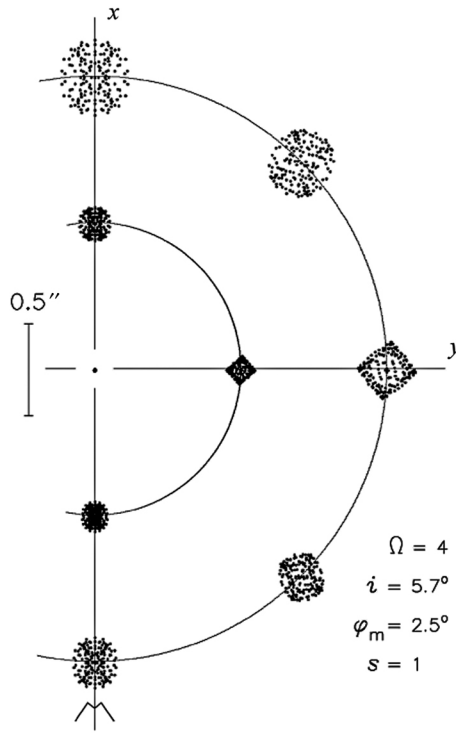
Figure 2: Best residual aberrations of an f/4 two-mirror reflective Schmidt ( \Omega = 4 ) in the non-centered system form. Inclination angle i = 5.7^\circ . Semi-FOV \varphi_m = 2.5^\circ . The under-correction parameter is just set to s = 1 . The radius of curvature of the spherical focal surface is also given by R_{\text{FOV}} = OF in eq. (3). The largest blur image corresponds to that with highest deviation of the FOV.
