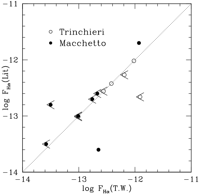
Fig. 6. Comparison of the H\alpha + [NII] flux measured in this work with the one measured by Macchetto et al. (1996) and by Trinchieri & di Serego Alighieri (1991) for 13 galaxies in common. Only 4 objects were detected by us, the remaining are upper limits.
