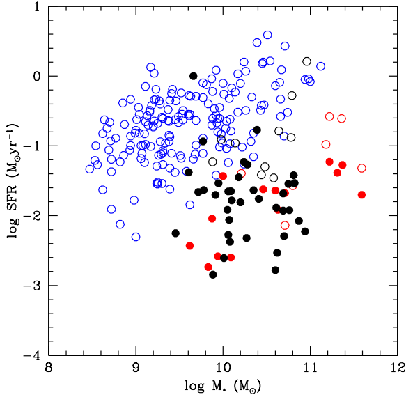
Fig. 9. Relation between the stellar mass and the SFR separately for a set of HRS galaxies (empty symbols): (blue: LTG, black: S0 + S0a, red: E) and the ETGs from this work (filled symbols): red: E; black: S0.
