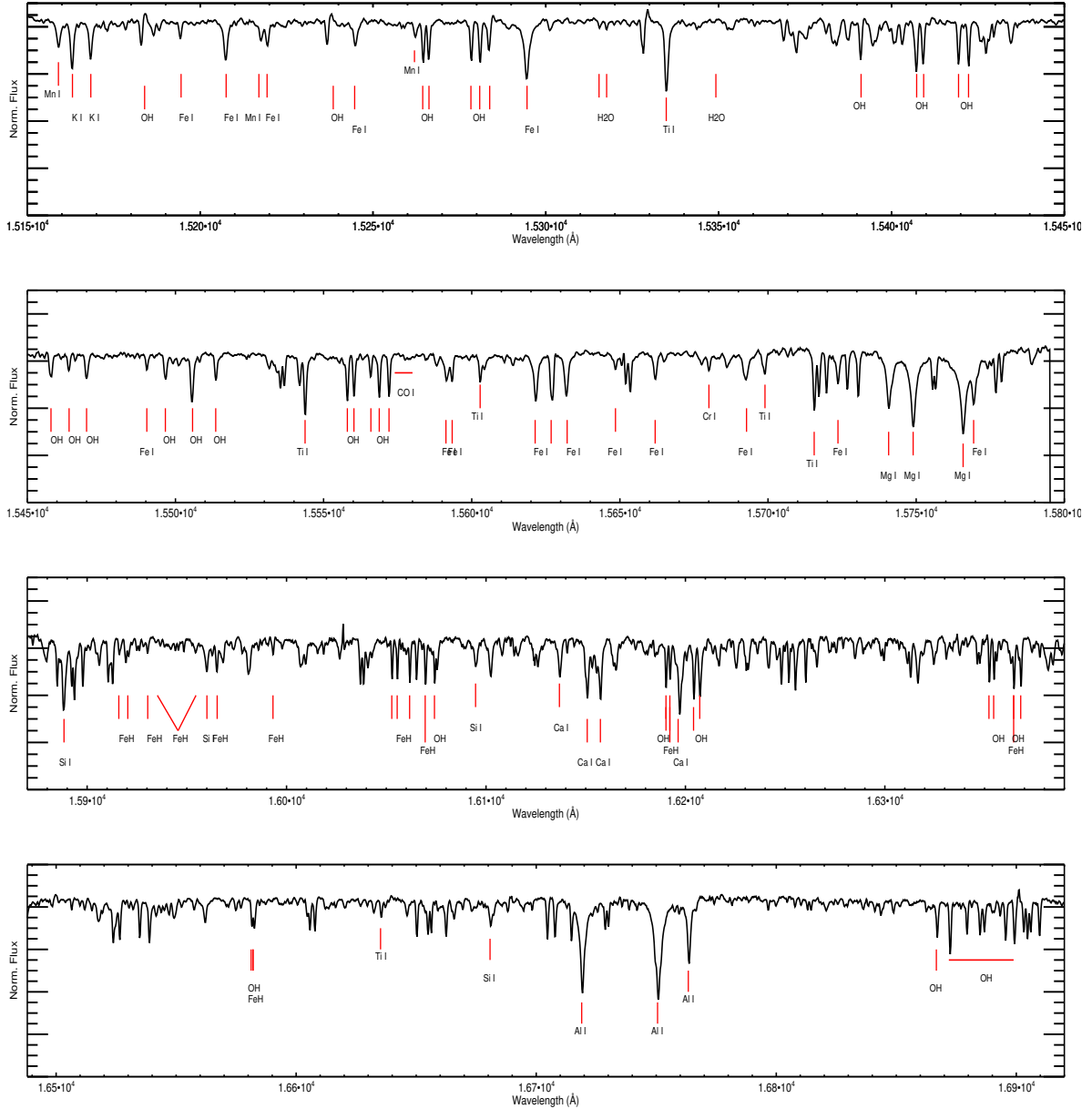
Fig. 1. APOGEE spectra of 2M11091225-0436249 (M0.5). The main spectral features can be seen, including atomic lines such as Fe I, Ca I, Na I, K I, Si I, Mg I, Al II, along with some hydride bands such as those of FeH and OH. We used mainly Souto et al. (2017) for the spectral feature recognition.
