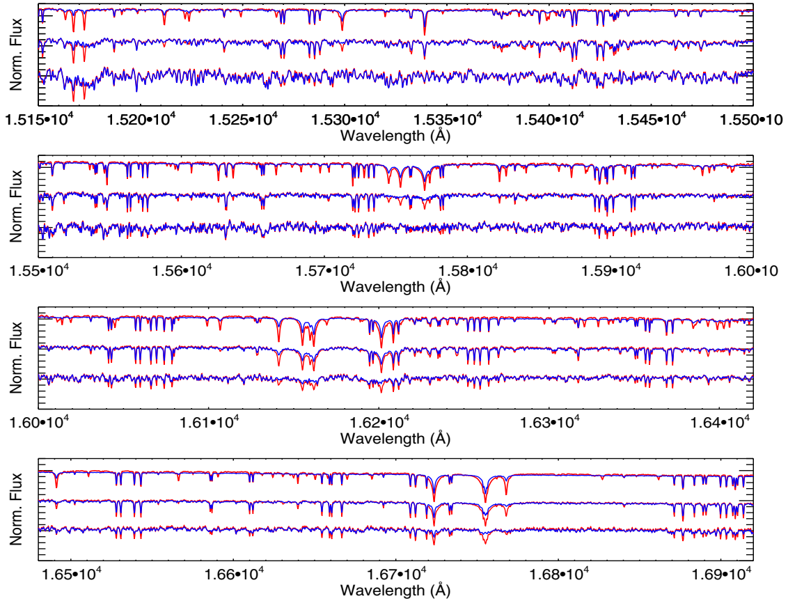
Fig. 2. BT-Settl synthetic spectra from 4000 K to 3000 K at a step of 500 K (top to bottom in each panel) of H -band computed with PHOENIX radiative transfer code. The red and blue lines represent the synthetic spectra at [\text{Fe}/\text{H}] = +0.5 (red) and -0.5 (blue) for T_{\text{eff}} = 4000 K, 3500 K, and 3000 K, at constant \log g of 5.5.
