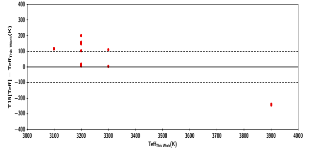
Fig. 7. Difference between the T_{\text{eff}} calibrations from Terrien et al. (2015, T15), estimated for the M dwarfs based on H -band relationships given by Newton et al. (2015), calibrations, and T_{\text{eff}} from this work. On the horizontal axis we show the T_{\text{eff}} that we infer from our best fit BT-Settl model used in this work. The black full line represents the origin and the dashed black lines represent the error from the grid size of 100 K.
