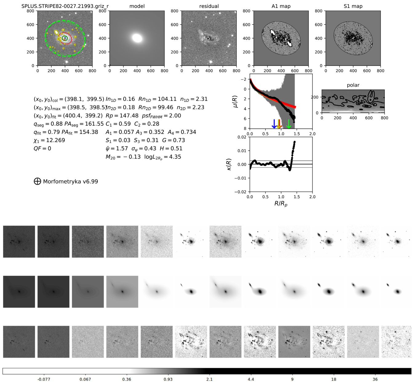
Figure 23. Upper panel: MORFOMETRYKA (top, from left to right): Original image; 2D Sérsic model image; the residual between image and model; asymmetry map used to compute A1; and smoothness map used to compute S1. Bottom: Various measurements (see text for details); Brightness profile (arbitrary units) and model fits; polar map used to compute image gradients and \sigma_{\psi} ; brightness profile curvature. Lower panel: MEGAMORPH-GALFITM: First row – galaxy images in the 12 S-PLUS bands ( u , J0378, J0395, J0410, J0430, g , J0515, r , J0660, i , J0861, and z , respectively); second row – galaxy models as fitted with GALFITM; third row – residuals. The colour bar shows relative intensity measurements with darkest colours indicating largest fluxes.
