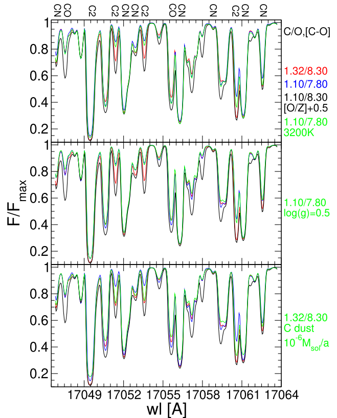
Figure 13. High-resolution R = 300\,000 spectra based on COMARCS models with T_{\text{eff}} = 3300 \text{ K} , \log(g [\text{cm s}^{-2}]) = 0.0 , and solar mass and metallicity having [O/Z] = +0.5 (black) and the standard composition ( [O/Z] = 0 ) with a constant C/O = 1.10 (blue) or [C-O] = 8.30 (red). They are compared to calculations (green) for [O/Z] = 0 and C/O = 1.10 , where T_{\text{eff}} was set to 3200 K (upper panel) or \log(g [\text{cm s}^{-2}]) to +0.5 (central panel). In addition, we show results with [O/Z] = 0 and [C-O] = 8.30 that have been obtained assuming an outer carbon dust shell computed for a mass-loss rate of 10^{-6} M_{\odot} \text{ a}^{-1} (green, lower panel). The data are normalized relative to their point with the largest flux. Absorption features produced by a single molecular species have been marked.
