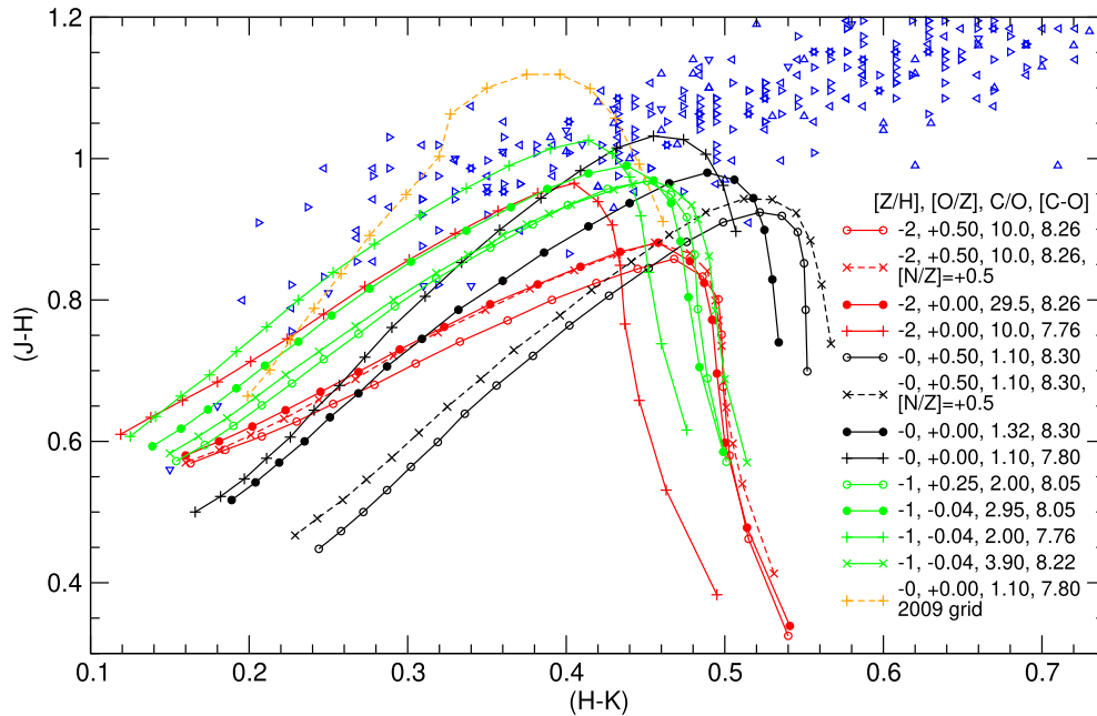
Figure 6. (J - H) versus (H - K) for temperature sequences of COMARCS models with \log(g \text{ [cm s}^{-2}\text{]}) = 0.0 and one solar mass. The shown abundance combinations and the corresponding colours and symbols are the same as in Fig. 5. In addition, we present results with [Z/H] = 0.0 and C/O = 1.10 taken from the previous COMARCS carbon star grid by Aringer et al. (2009), where the mass and surface gravity are identical (orange crosses, dashed line). The models are compared to observational data (blue triangles) listed in Bergeat, Knapik & Rutily (2001, up), Cohen et al. (1981, left), Costa & Frogel (1996, right), and Gonneau et al. (2016, down).
