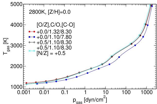
Figure 1. The effect of an increased oxygen and nitrogen abundance on the atmospheric temperature versus gas pressure structure is shown for different COMARCS models with T_{\text{eff}} = 2800 \text{ K} , \log(g [\text{cm s}^{-2}]) = 0.0 , and solar mass and metallicity. Results obtained adopting [O/Z] = +0.5 and [O/Z] = +0.5 , [N/Z] = +0.5 (cyan) are compared to calculations for the standard composition ( [O/Z] = 0 , [N/Z] = 0 ) with a constant C/O (blue) or [C–O] (red). The plot symbols placed along the curves mark steps of \Delta \log(\tau_{\text{Ross}}) = 0.5 starting with -5 at the outer edge.
