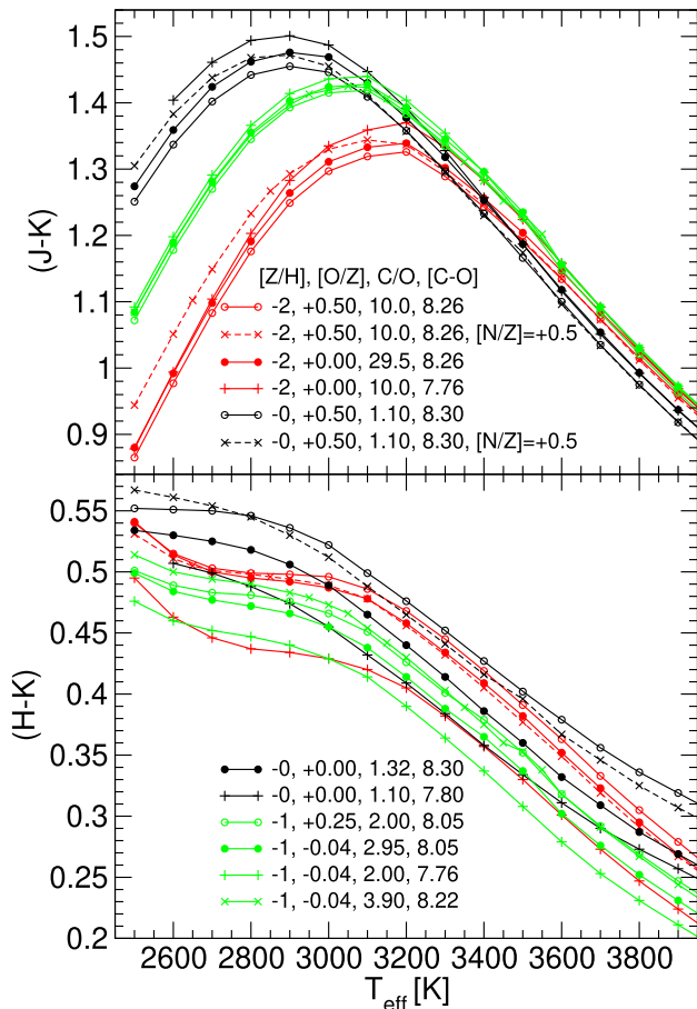
Figure 5. (J - K) and (H - K) as a function of the effective temperature for COMARCS models with \log(g \text{ [cm s}^{-2}\text{]}) = 0.0 and one solar mass. The colours correspond to different metallicities. For [Z/H] = 0 (black) and -2 (red) results obtained adopting [O/Z] = +0.5 (open circles) and [O/Z] = +0.5 , [N/Z] = +0.5 (x, dashed lines) are compared to calculations for the standard composition ( [O/Z] = 0 , [N/Z] = 0 ) with a constant C/O (plus) or [C-O] (filled circles). In the case of [Z/H] = -1 (green) we show oxygen-enriched models having [O/Z] = 0.25 , C/O = 2.0, and [C-O] = 8.05 (open circles) together with sequences where [O/Z] is set to -0.04 . They were created with the same C/O (plus), [C-O] (filled circles), and total amount of carbon \epsilon_C (x).
