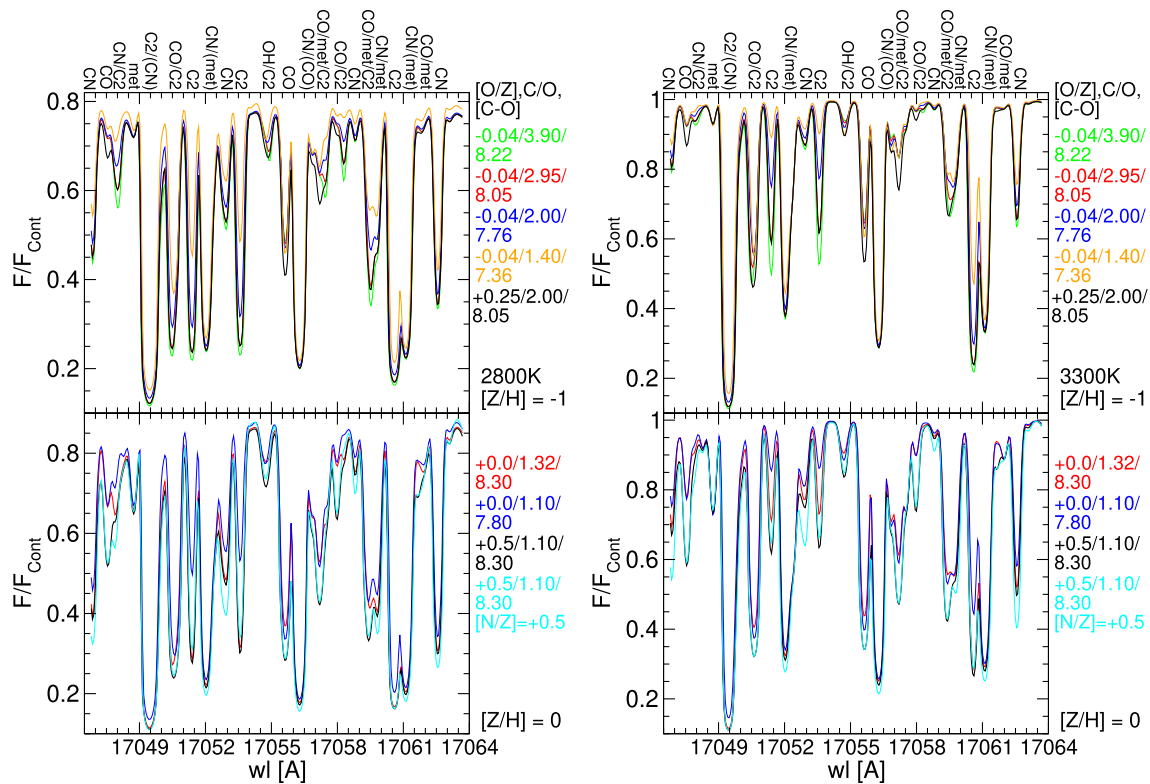
Figure 4. High-resolution R = 300\,000 spectra based on COMARCS models with \log(g [\text{cm s}^{-2}]) = 0.0 and one solar mass having T_{\text{eff}} = 2800 K (left-hand panels) or 3300 K (right-hand panels) and [Z/H] = 0 (lower panels) or -1 (upper panels). The data are normalized relative to a calculation without molecular and atomic line opacities. The different absorption features have been marked with the species creating them. ‘met’ stands for transitions due to metals. If a certain component of a blend is much weaker than the rest, it was put in brackets. For [Z/H] = -1 we compare an oxygen-enriched model ( [O/Z] = 0.25 , C/O = 2.0 , [C-O] = 8.05 , black) to calculations with [O/Z] = -0.04 having a constant C/O ( [C-O] = 7.76 , blue), [C-O] ( C/O = 2.95 , red), total amount of carbon \varepsilon_C ( C/O = 3.90 , [C-O] = 8.22 , green), and a lower C/O of 1.4 ( [C-O] = 7.36 , orange). For [Z/H] = 0 the shown abundance combinations and the corresponding line colours are the same as in Fig. 2.
