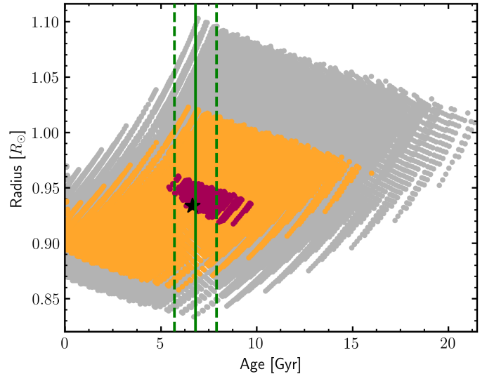
Fig. 5. Radius-age diagram of Kepler-82 from MESA stellar evolution models (MIST). The black star and the red, orange, and grey dots correspond to the best matching value and the 1\sigma , 2\sigma , and 3\sigma areas derived from results on the density of the whole data set photodynamical modelling and from the literature values of the effective temperature, the surface gravity, and the metallicity by Petigura et al. (2017). The gyrochronologic age is indicated in green by a solid line and its 1\sigma range as dashed lines.
