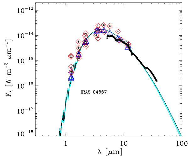
Figure 5. Examples of SED fitting for two dust-enshrouded stars. The observed photometry and the associated errors are marked with red diamonds and black bars, respectively. The IRS spectra are overplotted with black crosses. The synthetic photometry is plotted with blue triangles, the best-fitting spectrum is shown in solid black while the cyan lines are the acceptable spectra (see the text for more details).
