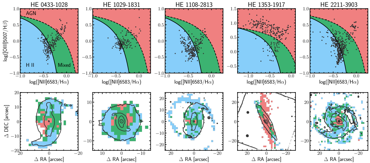
Fig. 2. Upper panel: MUSE BPT diagnostic diagrams with empirical dividing lines. The solid line shows data from Kauffmann et al. (2003) and the dashed line from Kewley et al. (2001) . The colors represent AGN ionization (red), ionization by H II regions (blue), and mixed regime (green). Lower panel: MUSE emission line 1.6'' × 1.6'' binned maps color-coded according to the BPT diagram regions; white-light contours are overlaid in black.
