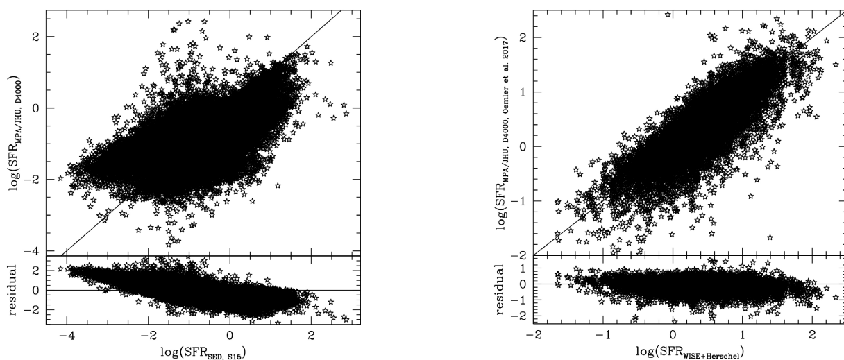
Figure A5. Comparison of the SFR based on the SED-based SFRs of Salim et al. (2016) and the D4000-based SFRs of the MPA-JHU catalogue corrected according to the calibration of Oemler et al. (2017).
