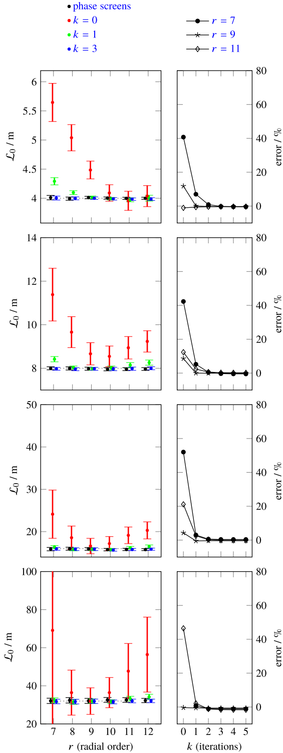
Figure 6. Outer scale estimations for \text{SNR}(r=9)=10 . Cf. Fig. 5 for details. The horizontal dotted line is the expected value \mathcal{L}_0 = 4 m (top), 8, 16, and 32 m (bottom).
