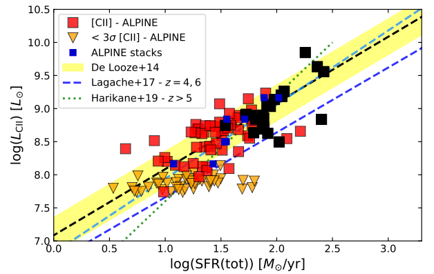
Fig. 4. Same as Fig. 2 using SFR(UV+IR). Here, SFR(IR) is derived from the observed UV slope and luminosity using the ALPINE IRX– \beta relation obtained from stacking (Fudamoto et al. 2020). The [C II]–detected galaxies follow the local relation well.
