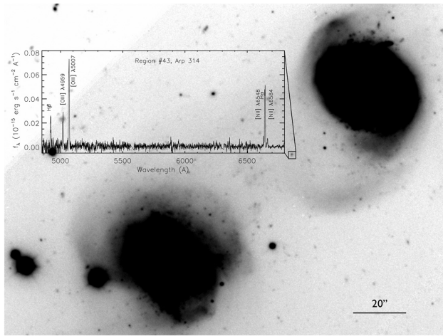
Figure 8. Gemini/GMOS r' -band image of Arp 314-1 and Arp 314-2. In this image, we show the location and spectrum of the region ID #43, which is located in the bridge that connects the main galaxies of this system.
