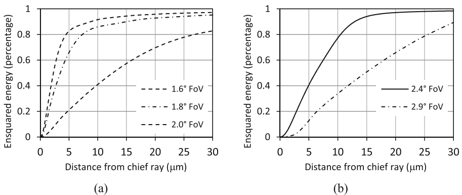
Fig. 6 Diffraction ensquared energy percentage as a function of the distance from the chief ray for the 1.6°, 1.8°, and 2.0° FoVs (a), and for 2.4°, and 2.9° FoVs (b) in the Metis UV channel
