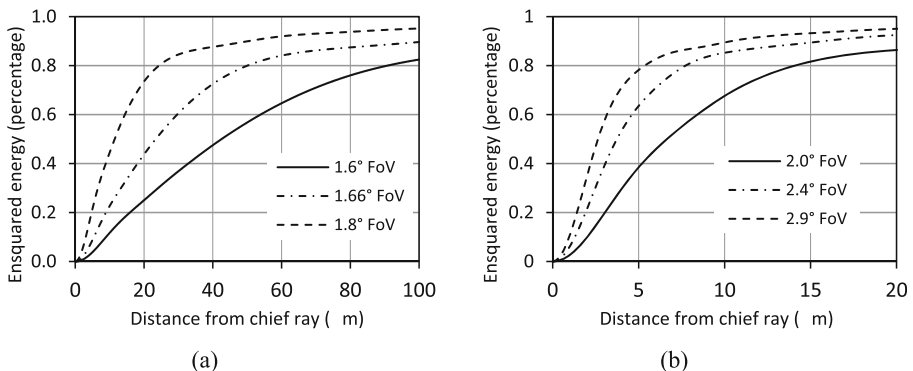
Fig. 9 Diffraction ensquared energy percentage as a function of the distance from the chief ray for the 1.6°, 1.66°, and 1.8° FoVs (a), and for 2.0°, 2.4°, and 2.9° FoVs (b) in the Metis visible channel
