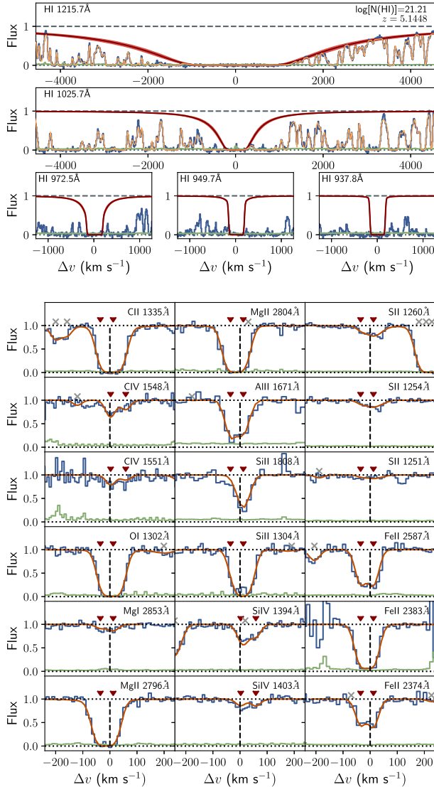
Figure 8. Model fits to the H I absorption and associated metal lines in the X-Shooter spectrum for the DLA system at z = 5.1448 . The data are shown by the blue stepped line in each panel, with the orange curve showing the overall fit within the wavelength range and, in the case of the Lyman series panels, the red curves show the individual strong H I system (with the width of the curves showing the extent given by the best fitting ranges quoted in Table 3). The upright triangles in each metal absorption panel identifies centroids of individual absorption components with the given velocity range of the DLA. The grey crosses indicate absorption features identified as not being at the same redshift (within the given velocity range) of the DLA.
