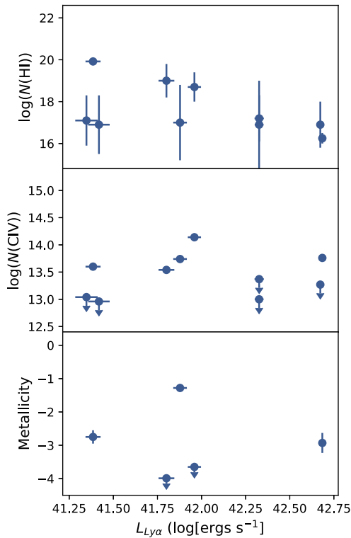
Figure 17. Absorption line properties as a function of nearest galaxy \text{Ly}\alpha luminosity, showing the H I column density (top panel), the C IV column density (middle panel), and the absorber metallicity (bottom panel).
