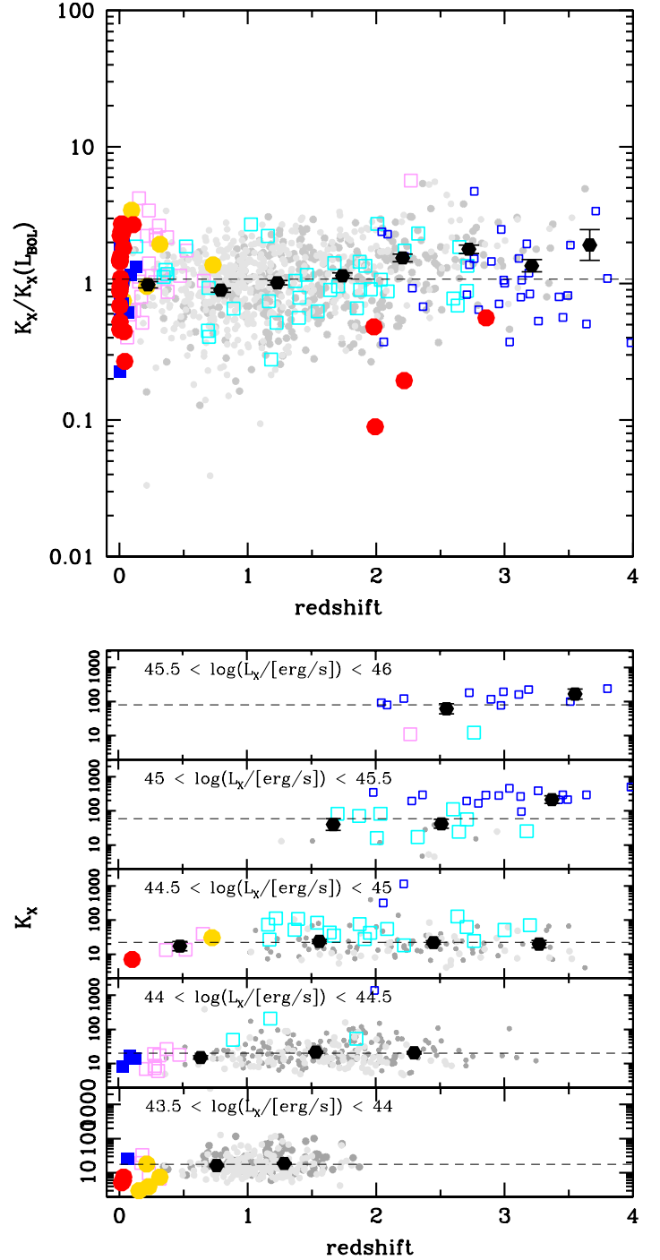
Fig. 8. Hard X-ray bolometric correction as a function of redshift. In the top panel , the normalized bolometric correction has been obtained by dividing K_X for the corresponding bolometric correction given by Eq. (2). Bottom panel : K_X as a function of redshift in five ranges of hard X-ray luminosity. Black hexagons are the average values of K_X computed in bins of redshift and the dashed line is the average K_X of the whole sample within the entire redshift range. Symbols are the same as in Fig. 6.
