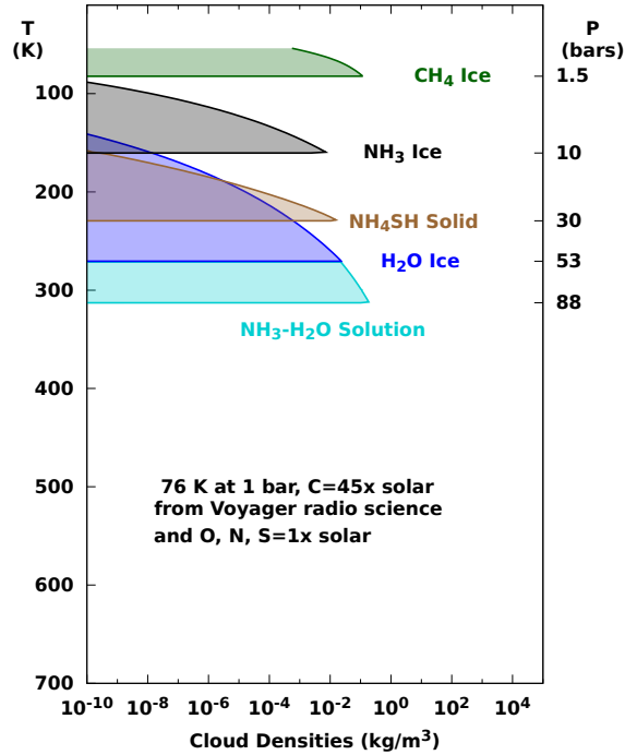
Figure 5. A solar-composition cloud structure model, constrained by the p-T and the \text{CH}_4 mole fraction ( \text{C}/\text{H} = 45\times solar) from Voyager [Lindal et al. 1987], would have an \text{NH}_3 -ice cloud layer but no \text{H}_2\text{S} -ice cloud. The results for Neptune are very similar, considering their temperatures are within a few degrees of each other at the 1 bar level. Cloud densities are calculated using the formula from Weidenschilling and Lewis (1973), which Wong et al. (2015) showed corresponds to a very large updraft length scale, equal to the pressure scale height H(z) at each altitude. Actual cloud densities in most Uranus/Neptune situations are likely to be much smaller than shown, but the pressure-levels of cloud bases are unaffected by the choice of updraft length scale.
