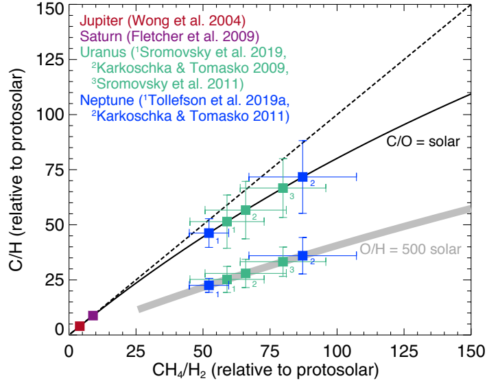
Figure 4. The C/H elemental ratio (y-axis) is non-linearly related to measured \text{CH}_4 hydrogen mixing ratios (x-axis), especially in compositions with high heavy-element abundances. The difference between solid and dashed lines accounts for the amount of hydrogen tied up in the volatile species \text{CH}_4 , \text{H}_2\text{O} , and \text{NH}_3 throughout the planetary envelope. In the C/O and C/N solar case (solid black line), the 87x solar \text{CH}_4 mixing ratio for Neptune (Karkoschka and Tomasko 2011) actually corresponds to a 72x solar C/H ratio (a 22% difference). In the 500x solar O/H case (Sec. 4.3.1), so much hydrogen is tied up in \text{H}_2\text{O} molecules that the observed \text{CH}_4 mixing ratio would imply only a 36x solar bulk C/H ratio in the envelope.
