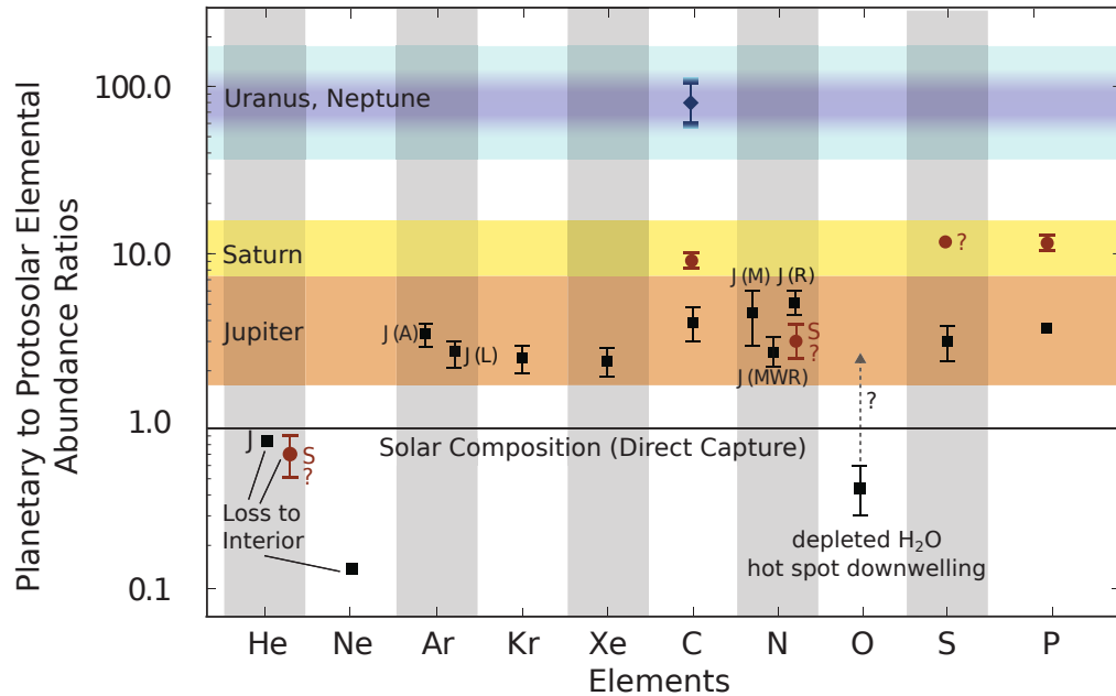
Figure 3. Elemental abundance ratios in the atmospheres of Jupiter, Saturn, Uranus and Neptune relative to the protosolar values. “N” in Jupiter represents values from ammonia ( \text{NH}_3 ) abundance measurements made by the Galileo probe mass spectrometer [J(M)] and the attenuation of probe radio signal [J(R)] as well as the Juno microwave spectrometer [J(MWR)]. The Jovian “Ar” value from the Galileo Probe measurements is shown as ratio to the protosolar Ar/H value of Asplund et al. [J(A)] and Lodders et al. [J(L)] since the solar argon values of the two sets of authors differ considerably. Saturn’s He and N are labeled S. N/H of Saturn is a lower limit, and S/H is highly questionable. Only C/H is determined for Uranus and Neptune from ground-based \text{CH}_4 to \sim 1 bar level, but could be greater in the deep atmosphere (see Atreya et al. (2019a) and references therein for other details). [This version of the figure was adapted from Fig. 2.1 of Atreya et al. (2019a), with permission from Cambridge University Press, PLSclear Ref No: 18694].
