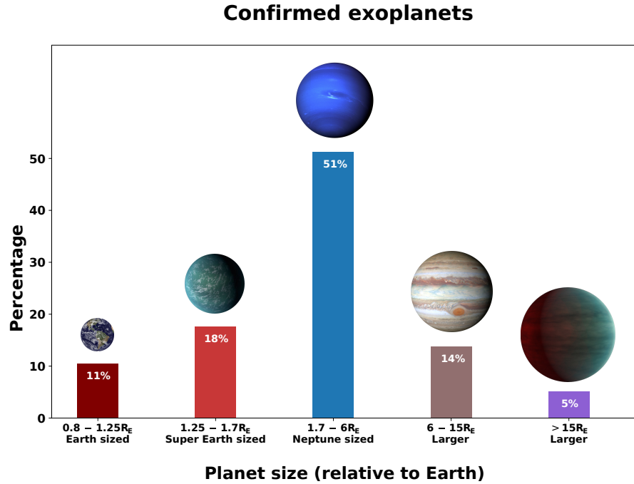
Figure 1. Mini-Neptune to Neptune-size exoplanets (1.7–6 R_E ) make up about one-half of nearly 3100 exoplanets with known radii out of a total of about 4000 confirmed exoplanets to date (2020 January). Percentages are rounded off to the nearest whole number; the actual values are 10.53%, 17.61%, 51.28%, 13.77% 5.08% and 1.73%, respectively, for 0.8–1.25 R_E , 1.25–1.7 R_E , 1.7–6 R_E , 6–15 R_E , >15 R_E and <0.8 R_E (not shown) size ranges. [Illustration based on listings in NASA Exoplanet Archive : https://exoplanetarchive.ipac.caltech.edu , and Extrasolar Planets Encyclopedia : http://exoplanet.eu ]
