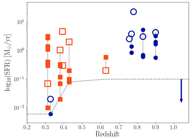
Figure 6. The star formation rate ( \text{SFR}_{\text{[O II]}} ) of the galaxies associated with absorbers as a function of redshift. The vertical grey lines connect galaxies associated with the same absorber. The open symbols indicate the galaxy at the smallest impact parameter. Absorbers selected based on their H I absorber are marked with orange squares, while metal-selected ones are marked with blue circles. The arrow marks the limits of the non-detection of the galaxy associated with the absorber Q1211z105. The dashed grey line represents the SFR limit at the redshift of the absorbers. We reach SFRs of 0.1 \text{ M}_{\odot} \text{ yr}^{-1} for most of the sample and lower (about 0.01 \text{ M}_{\odot} \text{ yr}^{-1} ) in case of deeper data (Q1130–1449).
