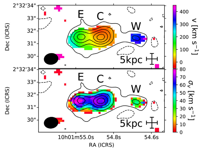
Figure 1. Total [C II] moment zero map (contours), velocity field (top colour), and velocity dispersion map (bottom colour). Contours begin at \pm 2\sigma , where 1\sigma = 0.1 \text{ Jy beam}^{-1} \text{ km s}^{-1} , and are in steps of 5\sigma . Zero velocity is defined as z_{[\text{C II}]} = 4.560 , or the redshift of the central source. The synthesized beam ( 1.07 \times 0.84 \text{ arcsec}^2 , with major axis position angle = -82^\circ ) is shown by the solid black ellipse to the lower left. A 5 \times 5 \text{ kpc}^2 scale is shown in the lower right. North is up and east is to the left.
