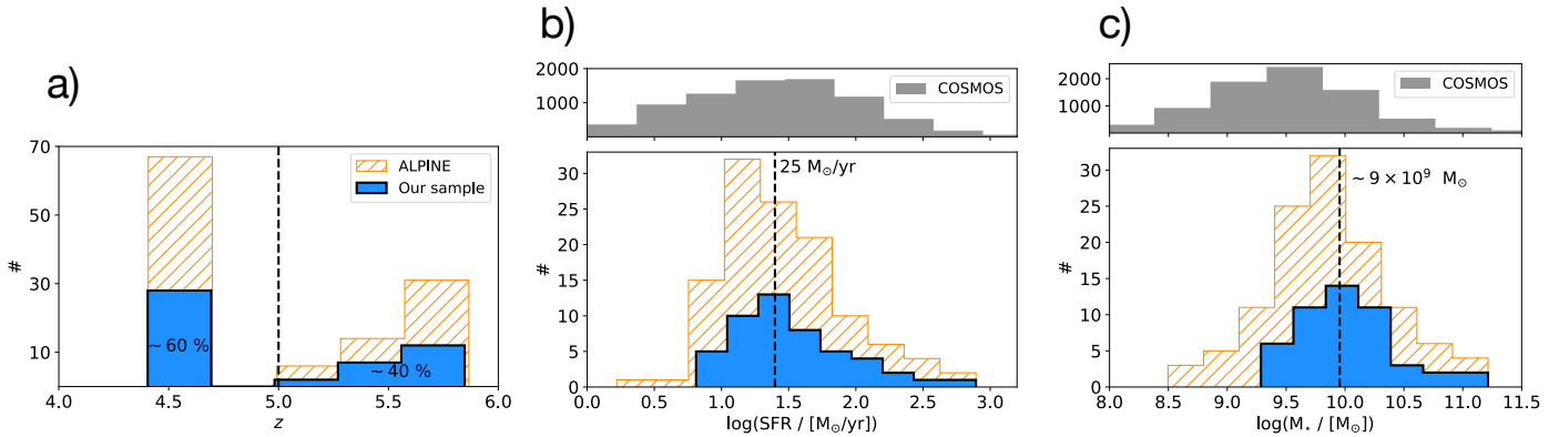
Fig. 1. Redshift (a), SFR (b), and M_* (c) distributions of galaxies in the ALPINE survey (orange) and galaxies in our final sample (blue), drawn from ALPINE and used in this work (see Sect. 3.1.2). For comparison, in panels b and c we show the SFR and M_* distributions of all COSMOS galaxies with photometric redshift in the ALPINE range z = [4.4-5.8] (from Laigle et al. 2016). The gap in the redshift distribution is due to the original ALPINE sample selection, tailored to avoid a prominent atmospheric absorption at \sim 325 GHz in ALMA band 7. The black dashed lines in panels b and c represent the median SFR and M_{\text{star}} of galaxies in our ALPINE-drawn sample.
