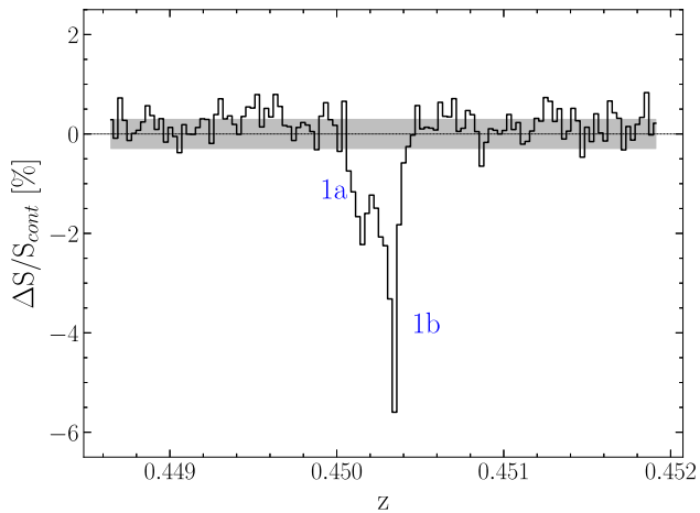
Figure 1. 21-cm HI absorption-line profile along the line of sight to the bright radio source PKS 1610-771. The light grey band indicates the 1\sigma limit in optical depth. There are two distinct velocity components (labelled 1a and 1b) that are 30 \text{ km s}^{-1} apart. The spectrum is reproduced from Sadler et al. (2020).
