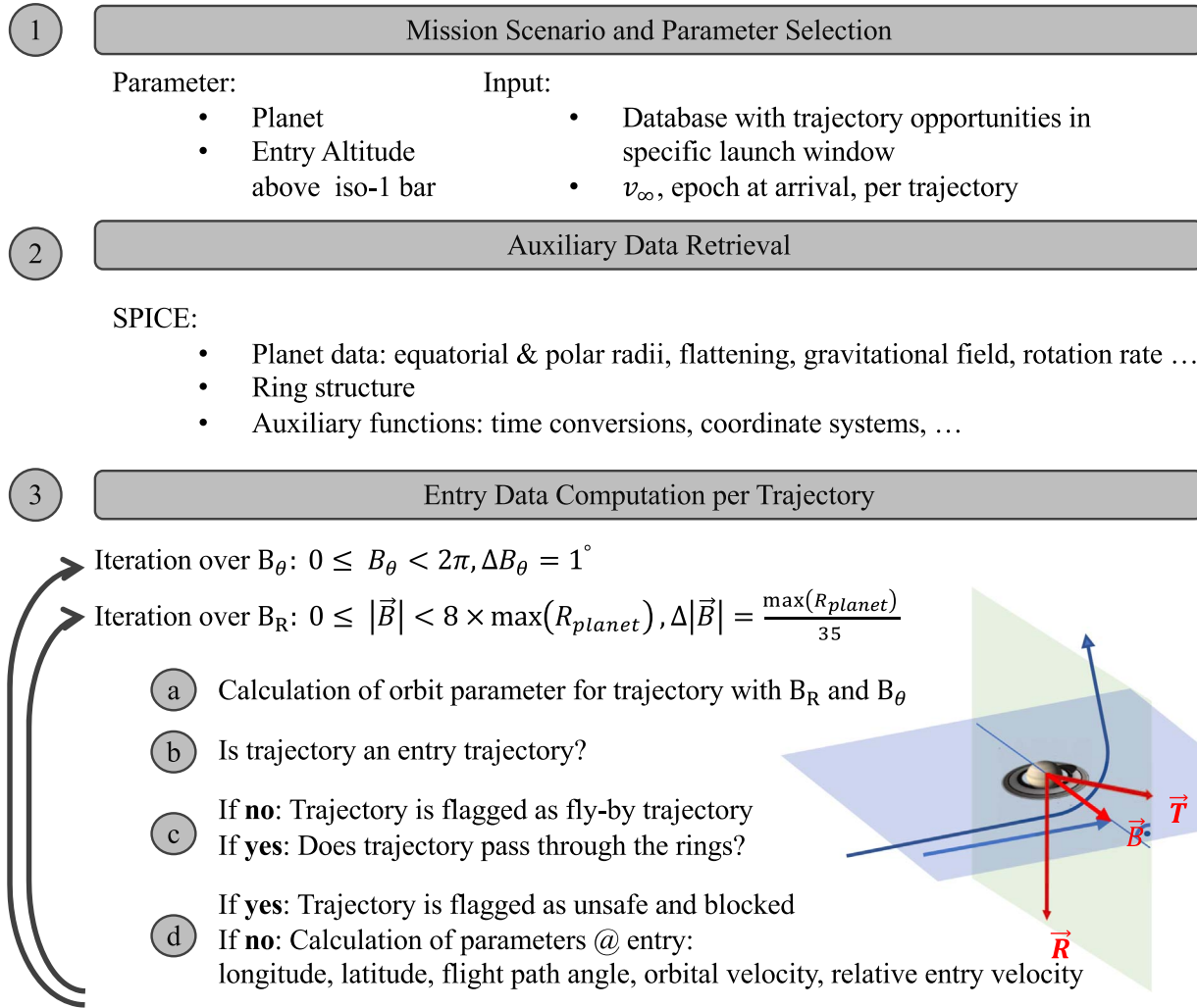
Figure 4. Flow chart sketching the logic of the entry data generation. After the (1) parameter and trajectory data set input and the (2) retrieval of the auxiliary data, the (3) entry data computation per trajectory is explained.
