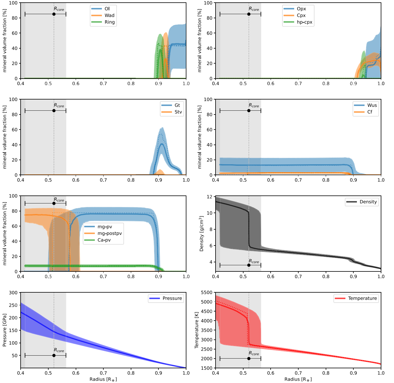
Figure B3. The uncertainty assessment of the modelled mineralogy and structure (taking K21-exoE as an example). The best-fitting mineralogy/structure profiles (corresponding to Fig. 5) are shown in dotted lines in each panel, with the 50th percentile and the range of 16th and 84th percentiles of the estimates shown in a solid line and a shadow area. The best-fitting profiles of pressure and density are exactly coincident with their 50th percentiles. The vertical dashed line in each panel indicates the 50th percentile of the core size ( R_{\text{core}} ), with its uncertainty shown in the light grey area. The illustration of the 50th percentile and the embraced range of [16th, 84th] percentiles of the lower mantle mineralogy has been cut off beyond the 1\sigma lower limit of the radius.
