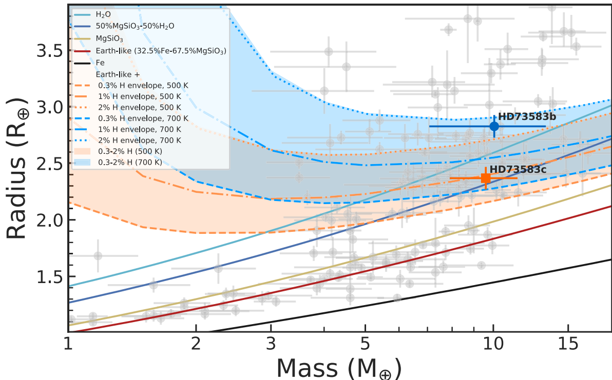
Figure 9. Mass versus radius diagram for small exoplanets ( 1 < R_p < 4 R_\oplus and 1 < M_p < 20 M_\oplus ). The grey points with error bars show planets with mass and radius measurements better than 30 per cent (As in the TEPCAT catalogue, https://www.astro.keele.ac.uk/jkt/tepcat/ , Southworth et al. 2007). HD 73583 b and c are shown with a (blue) circle and a (orange) square, respectively. The solid lines represent two-layer models as given by Zeng et al. (2016) with a different colour corresponding to a different mixture of elements. The non-solid lines correspond to rocky cores surrounded by an Hydrogen envelope with 0.3 per cent (dashed line), 1 per cent (dash-dotted line), and 2 per cent (dotted line) Hydrogen mass for exoplanets with equilibrium temperatures of 500 K (orange, similar to HD 73583 c's T_{eq} ) and 700 K (blue, similar HD 73583 b's T_{eq} ) as given by Zeng et al. (2019).
