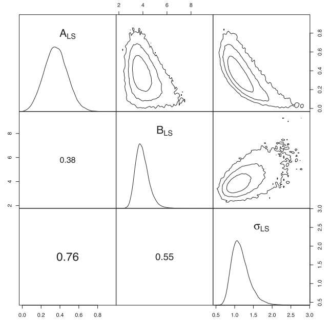
Figure 8. Scatterplot matrix for the fit of the bias corrected L_X^{\text{XXL}} - \sigma_v relation of the X-ray sample. The posterior densities are shown along the diagonal; the 1, 2, and 3\sigma confidence contours for the pairs of parameters are shown in the upper right panels. The lower left panels show the Pearson’s correlation coefficient for the corresponding pair of parameters (text size is proportional to the correlation strength).
