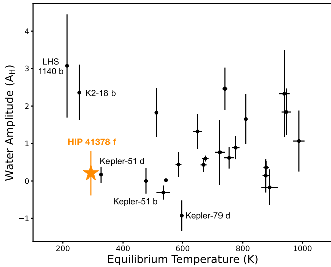
Figure 3. Equilibrium temperature vs. the 1.4\ \mu\text{m} \text{H}_2\text{O} feature amplitude ( A_H ) for the cooler ( T_{\text{eq}} < 1000\ \text{K} ) planets sample from Dymont et al. (2021) (points) and HIP 41378 f (orange star). There is no clear trend in A_H with planetary temperature.
