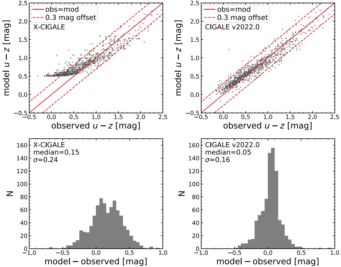
Figure 9. Top: model vs. observed u-z color of our SDSS quasars from X-CIGALE (left) and CIGALE V2022.0 (right). The red solid line indicates a model = observed relation; the red dashed lines indicate 0.3 mag offsets from this relation. We only plot points for sources having both u and z S/N > 5. Bottom: the distributions of model–observed u-z color from X-CIGALE (left) and CIGALE V2022.0 (right). The median and standard deviation values are labeled on each panel. The observed u-z color can be bluer than 0.5 mag. This cannot be reproduced with X-CIGALE, where the AGN disk SED shape is fixed, but CIGALE V2022.0 can account for these blue SEDs with u-z < 0.5 mag.
