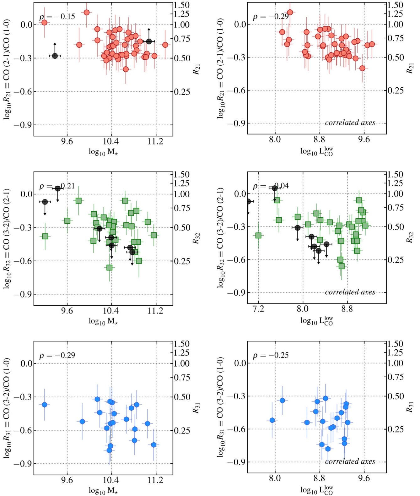
Figure 7. Correlations between line ratios and galaxy-integrated properties. Shown are the galaxy-integrated R_{21} , R_{32} , and R_{31} as a function of M_* and L_{\text{CO},\text{low}} . Each point represents one map pair for one galaxy, with the black points showing limits. Error bars reflect both statistical and calibration uncertainties. The numbers in the top left corners report the Spearman \rho relating the quantities on the x - and y -axes. As discussed in Section 4.2, the axes in the right column are correlated, and this may exert a significant effect on the observed relation. The correlations here appear even weaker than those in Figure 6, and we do not show any possible functional relations.
