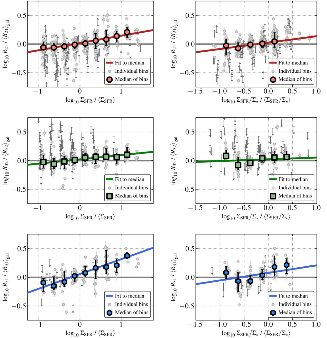
Figure 9. Correlations between line ratios and star formation activity. Each plot shows line ratio enhancement or deficit relative to the galaxy average, \log_{10} R/\langle R \rangle_{\text{gal}} , as a function of local SFR surface density and specific SFR. Before binning, we normalize \Sigma_{\text{SFR}} and \Sigma_{\text{SFR}}/\Sigma_* by their galaxy averages, so that the plots show how enhancements in the line ratio relative to the galaxy average correlate with enhancements in SFR or SFR/ M_* relative to the galaxy average. As in Figure 8, gray points show results for individual map pairs calculated as described in Section 3, and arrows show 4\sigma upper or lower limits. Colored points indicate the median result for all map pairs with a measurement in that bin, including limits, and so distill the general trend for the whole data set. The black vertical error bars show the 16th–84th percentile of individual measurements. The solid colored lines show a least-squares fit to all median values with at least five data points (see Table 5).
