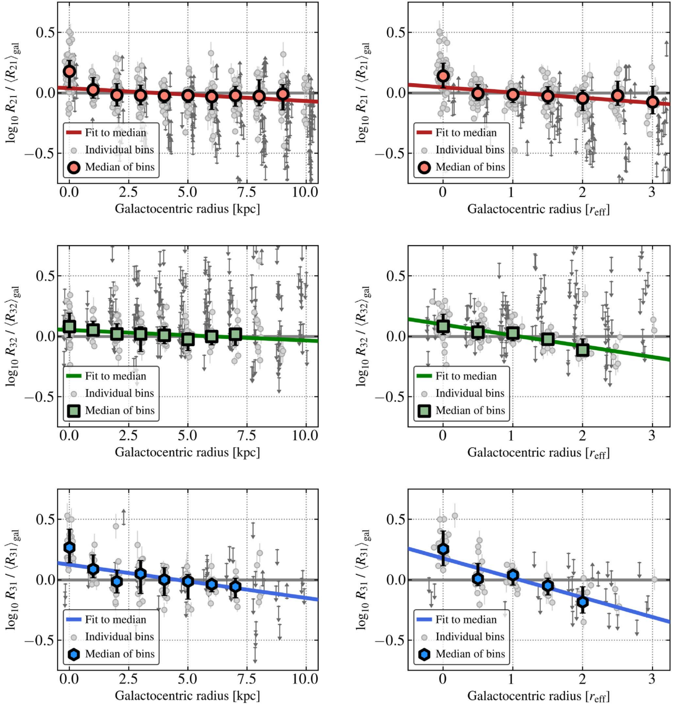
Figure 8. Correlations between line ratios and galactocentric radius. Each plot shows line ratio enhancement or deficit relative to the galaxy average, \log_{10} R/\langle R \rangle , as a function of galactocentric radius. Individual points showing binned results for individual galaxy plus survey pair combinations are calculated as described in Section 3. Arrows show 4\sigma upper or lower limits. Colored points indicate the median in each radial bin considering all galaxies and survey pairs with a measurement in that bin, including limits. The black vertical error bars show the 16th–84th percentile of measurement in that bin. We only plot median values, where a nonlimit 16%, 50%, and 84% value could be inferred from our measurements. The solid colored lines show a least-squares fit to all bins with at least five data points (see Table 5). The left panels show bins constructed considering physical radius, while the right panels normalize the radius by the half-mass radius, r_{\text{eff}} .
