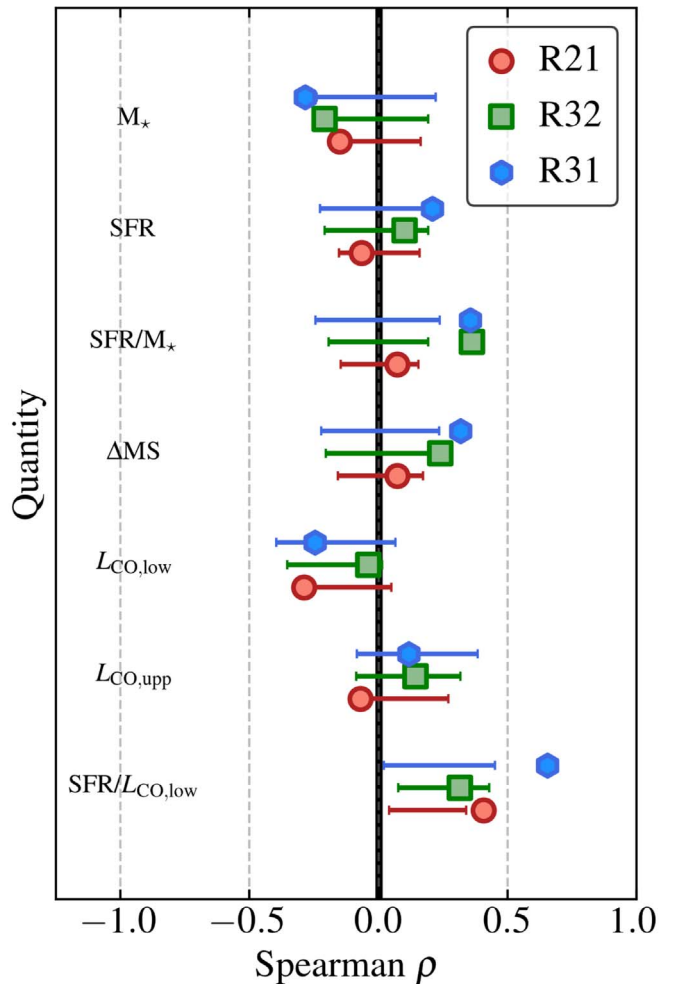
Figure 5. Rank correlation of line ratios with galaxy properties. Shown are the Spearman rank correlation coefficients relating global galaxy properties to measured line ratios, neglecting the limits. The bars show the 16%–84% range of coefficients expected under the null hypothesis of no real correlation (note that in the cases with correlated axes, the rank correlation coefficient for no true correlation may not be centered on zero; see the text). Here L_{\text{CO,low}} refers to the luminosity of the lower CO transition in the ratio, e.g., CO (1–0) in R_{21} , while L_{\text{CO,upp}} refers to the upper transition, e.g., CO (3–2) in R_{31} . As the contrast between results for L_{\text{CO,upp}} and L_{\text{CO,low}} demonstrates, the correlated axes play an important but hard-to-avoid role in determining correlations with L_{\text{CO}} and \text{SFR}/L_{\text{CO}} . Most correlations show marginal significance but are consistent with low-mass, high- \text{SFR}/M_{\star} , and high- \text{SFR}/L_{\text{CO}} galaxies showing higher line ratios, especially among the measurements involving CO (3–2). See also Figure 6.
