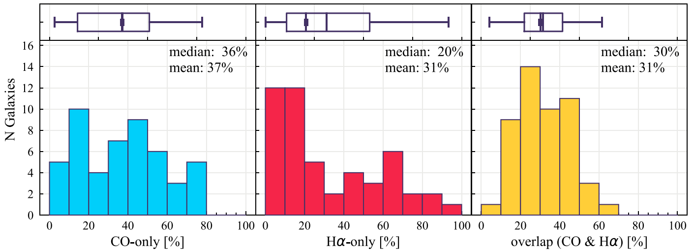
Figure 3. Distribution of global CO-only (left), H \alpha -only (middle), and Overlap (right) sight-line fractions at a resolution of 150 pc. Corresponding box plots are shown at the top of each panel. The boxes show the interquartile ranges (IQR; the Q1/25 percentile to Q3/75 percentile), and the horizontal whiskers extend to Q1 - 1.5 \times \text{IQR} and Q3 + 1.5 \times \text{IQR} . The inner vertical belt-like symbol and line in the boxes represent the median and mean of the distribution, respectively; the values are also given in the upper right of each panel. Substantial galaxy-to-galaxy variations are seen for all sight-line categories.
