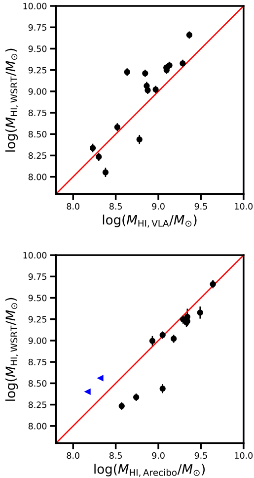
Fig. 4. A comparison of HI masses recovered by our WSRT survey and the VLA measurements of Bravo-Alfaro et al. (2000, 2001), and the Arecibo survey of Gavazzi et al. (2006) in the top and bottom panels, respectively. Red lines in both figure represent a 1:1 relation. Blue triangles in the bottom panel indicate M_{\text{HI}} upper limits in the Gavazzi et al. (2006) catalogue.
