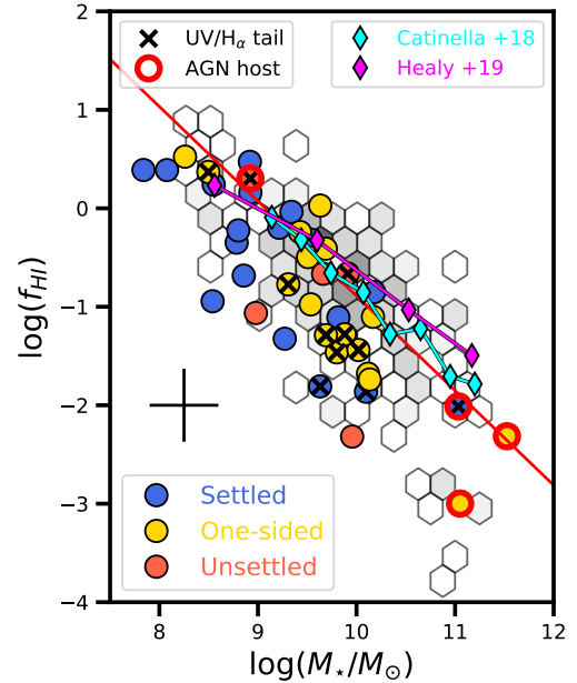
Fig. 8. Distribution of HI-selected Coma galaxies (coloured circles) and the field galaxy reference sample (hexagonal bins) in the stellar mass – atomic gas fraction plane. Red line shows our best-fit linear relation to the SFMS galaxies (defined using Fig. 7) in the reference sample. Black crosses mark Coma galaxies with tails at H_\alpha or UV wavelengths, while red circles denote ongoing AGN activity. Black errorbars are the mean uncertainties of the Coma measurements. The cyan and magenta diamonds indicate the median gas fractions measured by Catinella et al. (2018) and Healy et al. (2019), respectively.
