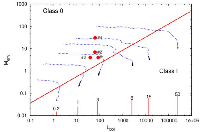
Figure 21. The (L_{\text{bol}}, M_{\text{env}}) diagram of the candidate protostars detected in the western clump (ID numbers are the same as in Figure 19). The dashed blue lines represent the evolutionary tracks from André et al. (2008). Evolution proceeds from the upper left to the lower right (indicated by arrows at the end of each track). The final stellar masses of these tracks, in solar units, are given above the vertical lines. The slanted red line corresponds to the location where 50% of the initial core mass is converted into stellar mass (Bontemps et al. 1996; André et al. 2000).
