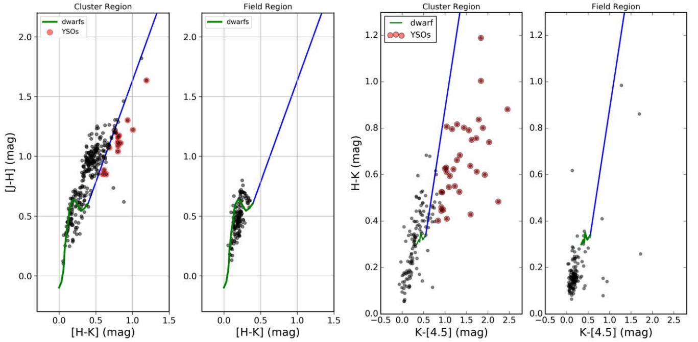
Figure 9. Left: the (J-H, H-K) CC diagram for the cluster region and the control field region. The green curves are the intrinsic dwarf locus from Bessell & Brett (1988). Right: the (H-K, K-[4.5]) CC diagram for the cluster region and the control field region. The green curves are the intrinsic dwarf locus of late M-type dwarfs (Patten et al. 2006). In all of the plots, the blue lines represent the reddening vectors drawn from the location of an M6 dwarf, while the red circles represent likely NIR excess sources.
