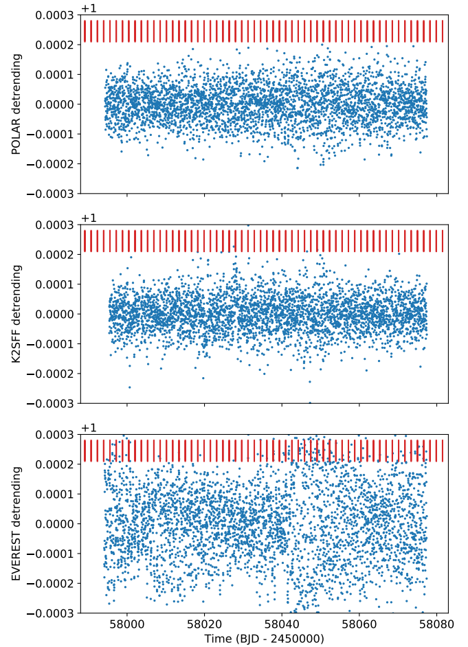
Fig. 1. Normalized flux from K2 photometry with systematics corrected via the POLAR pipeline (top panel), K2SFF pipeline (middle panel), and EVEREST pipeline with a Savitzky–Golay filtering (bottom panel). The red lines indicate the expected transit positions for the short-period planet (HD 137496 b).
