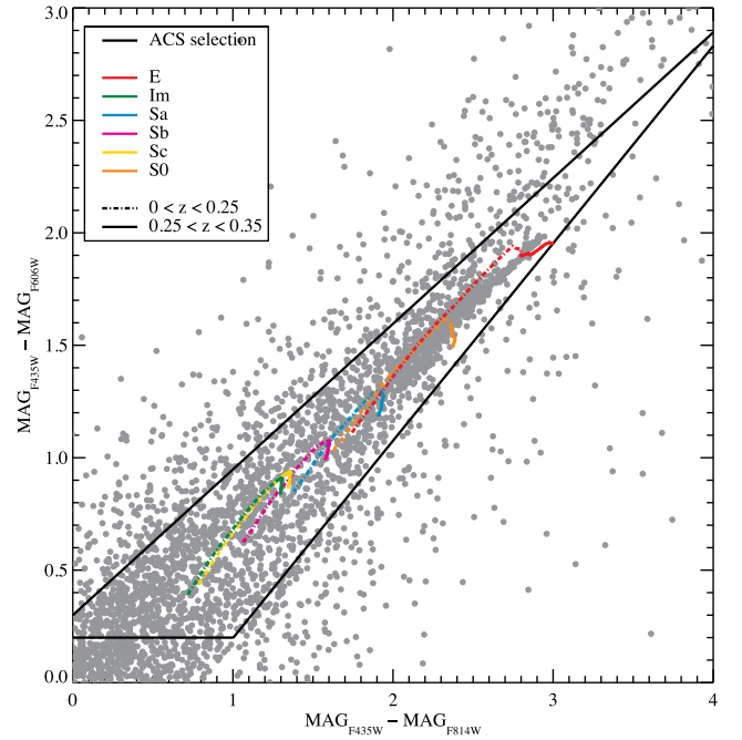
Figure 3. Colour–colour diagram (\text{mag}_{\text{F435W}} - \text{mag}_{\text{F814W}}) versus (\text{mag}_{\text{F435W}} - \text{mag}_{\text{F606W}}) as in Fig. 1. The solid black lines delineate the colour-cut defined for this work. The different spectral templates from Coleman et al. (1980) and Kinney et al. (1996) as well as theoretical models from Bruzual & Charlot (2003) are marked by different colours: elliptical galaxies (red); Magellanic irregulars (green); spiral Sa galaxies (cyan); spiral Sb (magenta); spiral Sc (yellow); and S0 galaxies (orange). The dash-dotted curves correspond to a redshift range 0 < z < 0.25 (foreground galaxies), the solid ones to 0.25 < z < 0.35 (cluster members).
