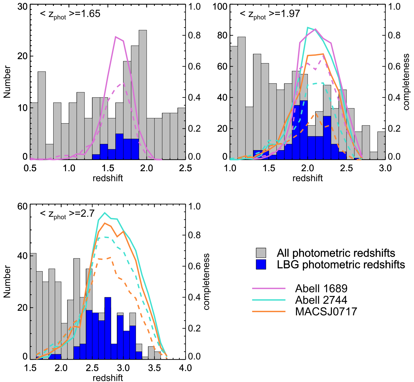
Figure 14. Photometric redshift distribution of LBGs. The gray histogram shows the photometric redshift distribution of all objects in the fields. The blue histogram highlights the photometric redshift distribution of those galaxies selected as LBGs. The solid and dashed lines show the simulated completeness distribution over redshift for a galaxy with \mu_{\text{mag}} = 1.0 and m_{\text{UV}} = 27 and 28 , respectively. The purple, blue, and orange colors present the completeness distribution for A1689, A2744, and MACSJ0717, respectively. The right-hand axis shows the completeness values.
