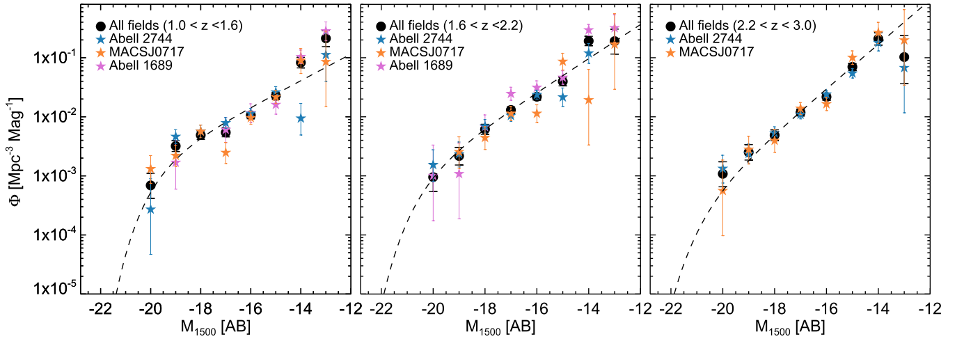
Figure 6. Rest-frame UV luminosity function for each lensing cluster at 1.0 < z < 1.6 , 1.6 < z < 2.2 , and 2.2 < z < 3.0 in the left, middle, and right panels, respectively. The purple, blue, and orange stars show the binned LF of A1689, A2744, and MACS J0717, respectively. The black circles are the binned LFs after combining all of the three lensing clusters. The dashed line is the best-fit Schechter function (see Section 8.2).
