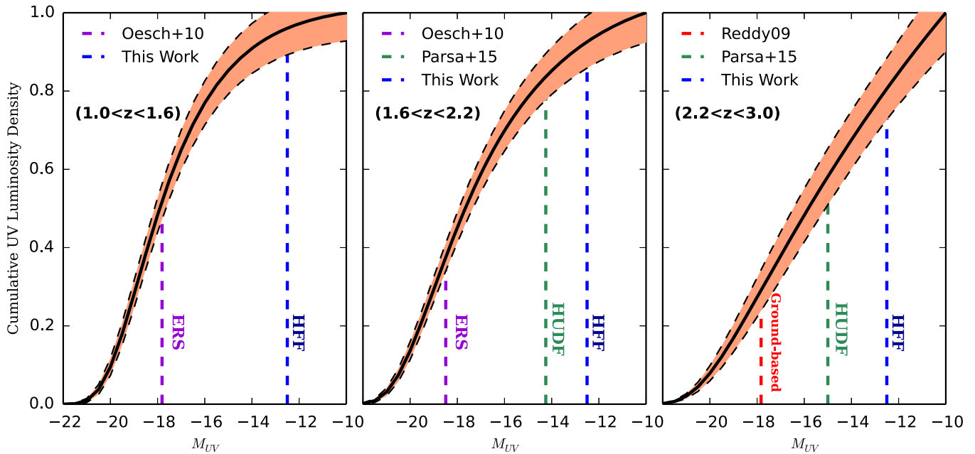
Figure 11. Cumulative UV luminosity density at 1.0 < z < 1.6 (left), 1.6 < z < 2.2 (middle), and 2.2 < z < 3.0 (right). The purple, green, and blue dashed lines show the UV-limiting magnitudes for the ERS (Oesch et al. 2010a), Hubble Ultra Deep Field (Parsa et al. 2016), and our samples. The orange region represents the 1\sigma uncertainty measured at each M_{UV} . We have measured the LF of galaxies responsible for 58%, 55%, and 59% of total UV luminosity density at z \sim 1.3 , z \sim 1.9 , and z \sim 2.6 , respectively.
