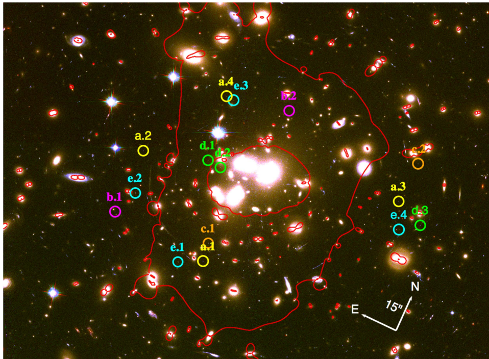
Figure 16. The color image is a composite of the F475W (blue), F625W (green), and F814W (red) filters. The contours show the critical lines for sources at z = 2.5 . The circles denote the positions of the newly found multiple images. A compass provides the orientation, and the lengths of the arrows show the 15'' scale. Some of the labels have been offset slightly.
