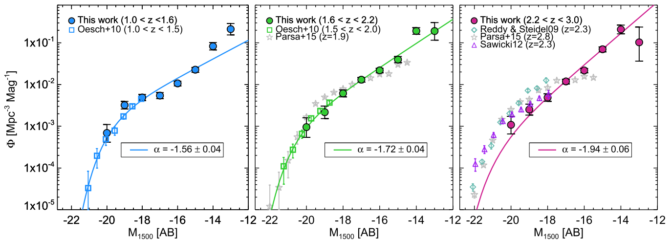
Figure 7. Rest-frame UV luminosity functions at z \sim 1.3 (left), z \sim 1.9 (middle), and z \sim 2.6 (right). The blue, green, and red circles are our binned LFs combining all three lensing clusters (see Section 8.1). The blue and green squares are the LFs from Oesch et al. (2010a) at 1.0 < z < 1.5 and 1.5 < z < 2.0 , respectively, where the individual data were used for our MLE fitting. The light blue diamonds are the LFs from Reddy & Steidel (2009) based on a BX-selected sample of star-forming galaxies. The gray stars and purple triangles are the results from Parsa et al. (2016; photometric redshift selection) and Sawicki (2012; BX selection), respectively. The solid line in all three panels shows our best Schechter fit through a MLE technique.
