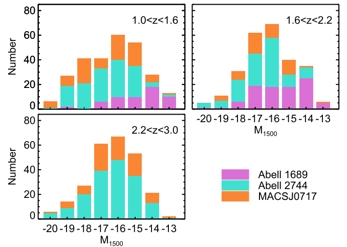
Figure 3. Intrinsic absolute UV magnitude (i.e., corrected for the lensing magnification) distribution of all galaxies in our three redshift slices. The colors are similar to Figure 2, and they show the number of candidate galaxies for each absolute magnitude bin. We cover a large luminosity range by combining the HFFs with A1689, which finds the faintest galaxies ( M_{1500} > -14.5 ).
