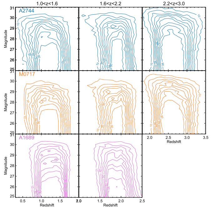
Figure 4. Completeness as a function of intrinsic apparent magnitude on the y-axis and redshift on the x-axis. The blue, orange, and purple contours show the completeness simulation values for A2744, MACS J0717, and A1689, respectively. The left, middle, and right columns represent the completeness contours for photometric redshift samples at 1.0 < z < 1.6 , 1.6 < z < 2.2 , and 2.2 < z < 3.0 , respectively. These contours are drawn for a magnification of \mu_{\text{mag}} = 2.0 magnitudes.
