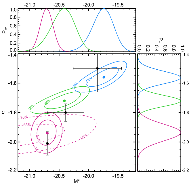
Figure 8. 68% and 95% contours of the z \sim 1.3 , z \sim 1.9 , and z \sim 2.6 photometric redshift LFs shown with blue, green, and red colors, respectively. The red dashed line shows the contours for the z \sim 2.6 LF before adding the M^* prior (see Section 8.2). The marginalized probability distribution of each parameter P(\alpha) and P(M^*) are also plotted on the right and top sides, respectively. The best-fit values of Schechter parameters for each LF is shown with a filled circle. The black filled circles with error bars denote the best-fit values for the LBG LFs (see Section 9).
