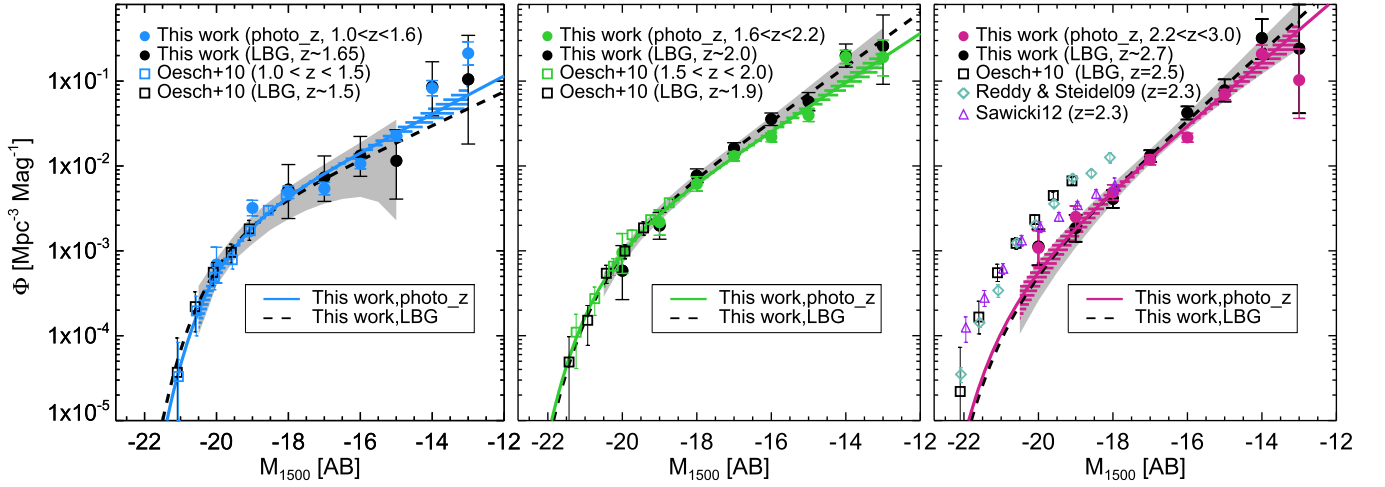
Figure 9. Comparing the UV LF of the LBG and photometric redshift samples. The black filled circles are the binned LBG LF for our F225W-, F275W-, and F336W-dropout samples from the left to right panels, respectively. The black dashed line in each panel represents the best-fit Schechter function for the corresponding LBG LF. The gray regions indicate the \pm 2\sigma confidence region for each fit derived via Monte Carlo simulation. We overplot the binned and best-fit LFs derived from our photometric redshift samples as shown before in Figure 7. The hatched region denotes the \pm 2\sigma confidence region of the best-fit photometric redshift LF. The black open squares are the binned LBG LFs from Oesch et al. (2010a). The rest of the colors and symbols are as in Figure 7. For each redshift range, our binned and best-fit LFs are consistent within the 2\sigma error bars.
