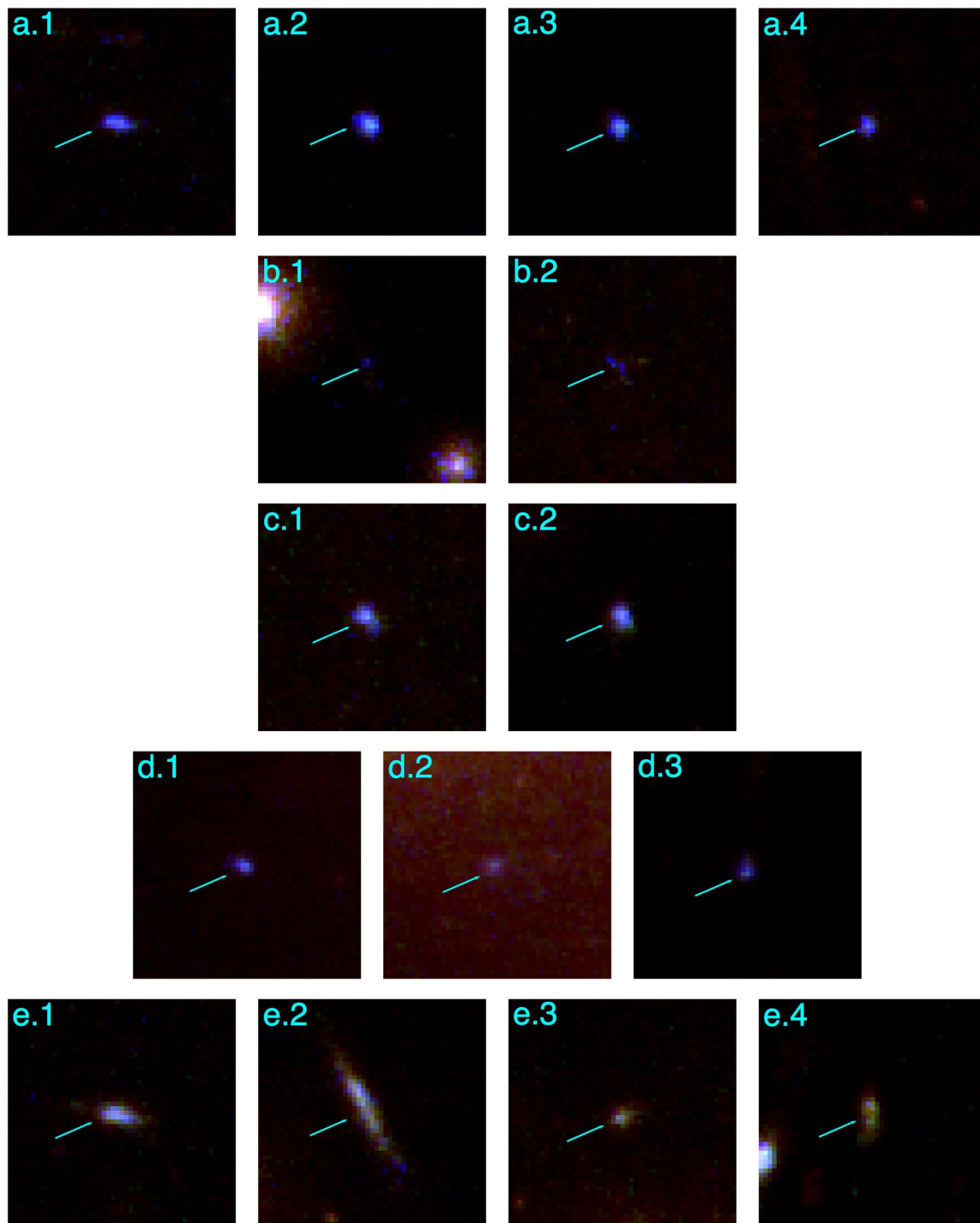
Figure 15. Newly identified multiply imaged systems in A1689. The arrow in each stamp denotes the position of each multiple image. The color image is a combination of the F475W (blue), F625W (green), and F814W (red) filters. We note that the reddening in the d.2 image is due to a nearby cluster member. The size of each cutout is 2'' .
