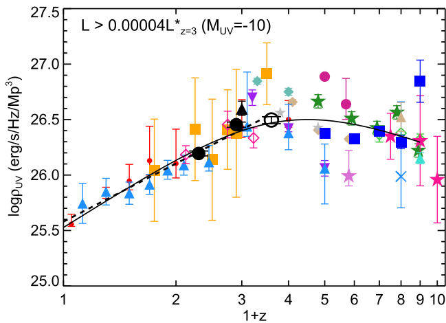
Figure 12. Redshift evolution of the unobscured UV luminosity density measured at rest-frame wavelength of 1500 Å. To estimate the \rho_{UV} values, the LFs are integrated down to M_{UV} = -10 at all redshifts. The uncertainty for each data point is derived by retaining the fractional error of published \rho_{UV} values from each author. The black filled circles are derived from our photometric redshift LF estimates. Similar to Figure 10, we show our \rho_{UV} measurement at z = 2.6 with a black open circle as it depends on the choice of M^* prior. The rest of the symbols are similar to Figure 10, except the red filled circles which are from Schiminovich et al. (2005) using the LF estimates from Arnouts et al. (2005) and Wyder et al. (2005) (shown with red filled circle and blue asterisk in Figure 10, respectively). The dashed line indicates the best-fitting power law to the data points at z < 2.6 . The solid line shows the best-fitting function (see Equation (12)) for the redshift range of 0 < z < 8 .
