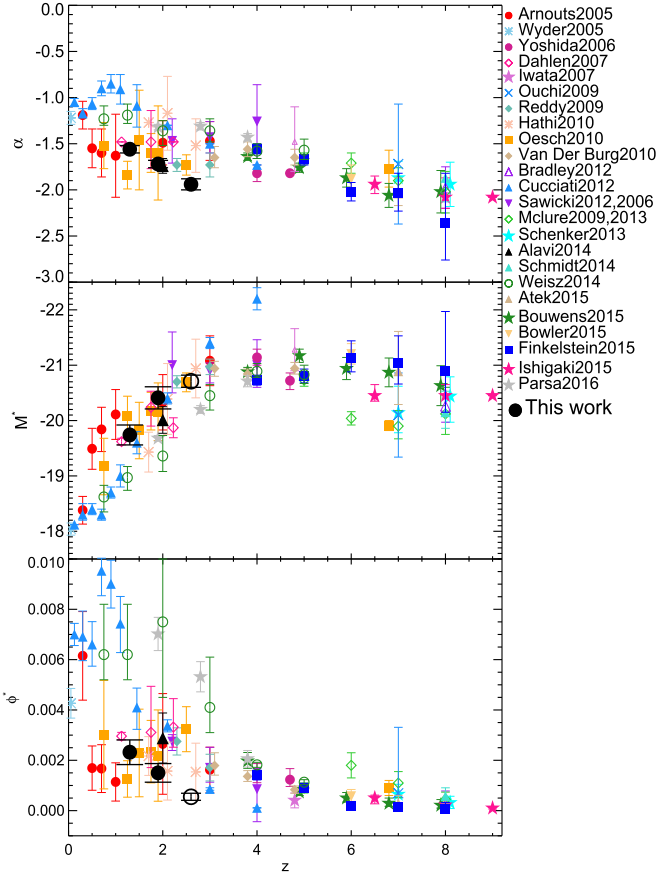
Figure 10. Redshift evolution of the Schechter parameters \alpha (top), M^* (middle), and \phi^* (bottom). The present determinations are shown with black filled circles. Our measurements of M^* and \phi^* at z \sim 2.6 are shown with black open circles, as they are dependent on our choice of the M^* prior. All symbols from the literature are summarized in the right-hand side of the plot. A detailed description of each parameter evolution is given in the text (see Section 10.2).
