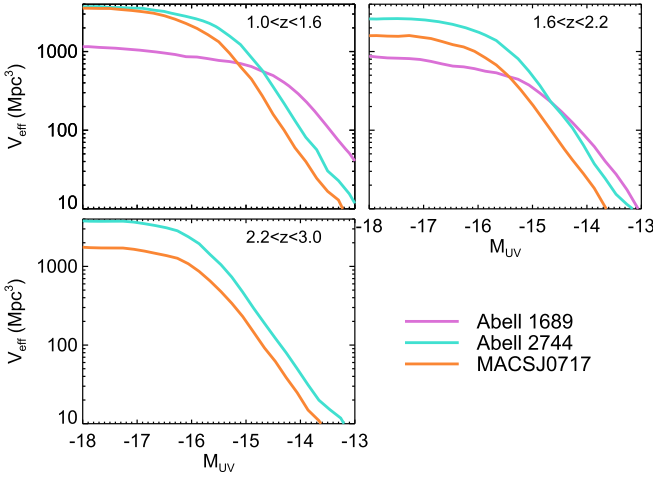
Figure 5. Effective volume estimates at each redshift slice in each field. The HFF clusters provide a large volume over faint magnitudes ( M_{UV} < -15.5 ), while the A1689 cluster enables even fainter galaxies ( M_{UV} > -14.5 ) beyond the HFF magnification limits to be probed.
