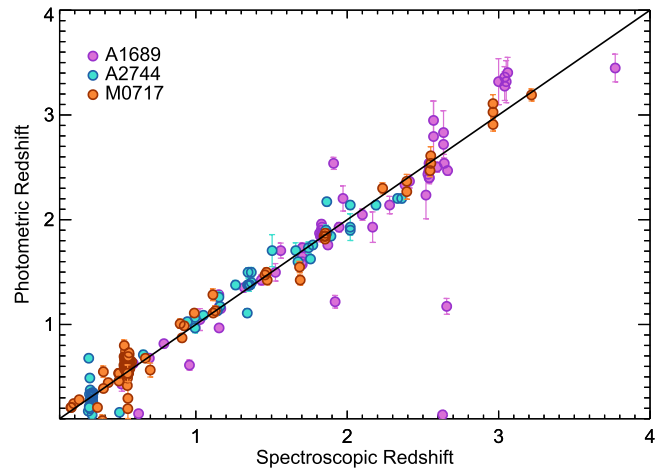
Figure 1. Comparison between the photometric and spectroscopic redshifts for 244 galaxies in all three lensing fields. The spectroscopic redshifts are either from our Keck/MOSFIRE and Keck/LRIS data or from the literature (for more details, see the text). The purple, orange, and cyan circles show the measurements for the A1689, MACSJ0717, and A2744 cluster fields, respectively.
