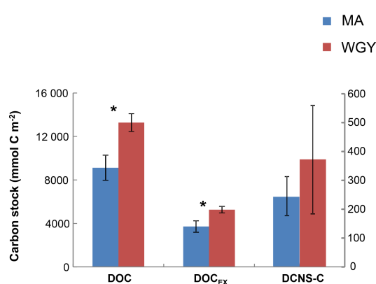
Figure 6. Integrated carbon stocks ( \text{mmol C m}^{-2} ) over the euphotic zone carbon in terms of DOC, DOC EX and DCNS-C (secondary axis). * DOC and DOC SL were statistically different between MA and WGY areas (Mann–Whitney test, p < 0.05 ).
