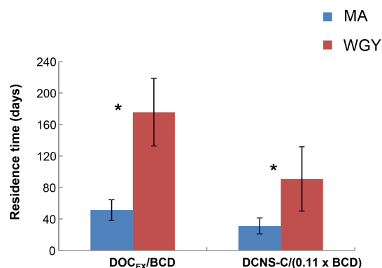
Figure 7. Residence time (days) of semi-labile DOC ( T_{r\text{ SL}} ) and DCNS-C ( T_{r\text{ DCNS-C}} ) for MA and WGY areas. * T_{r\text{ SL}} and T_{r\text{ DCNS-C}} were statistically different between MA and WGY areas (Mann–Whitney test, p < 0.05 ).
